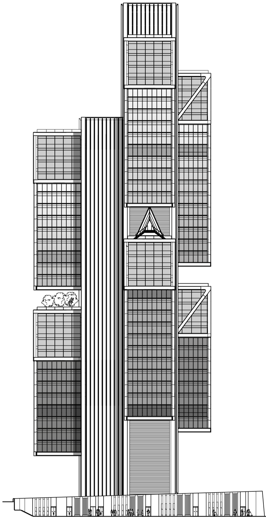
East Elevation
