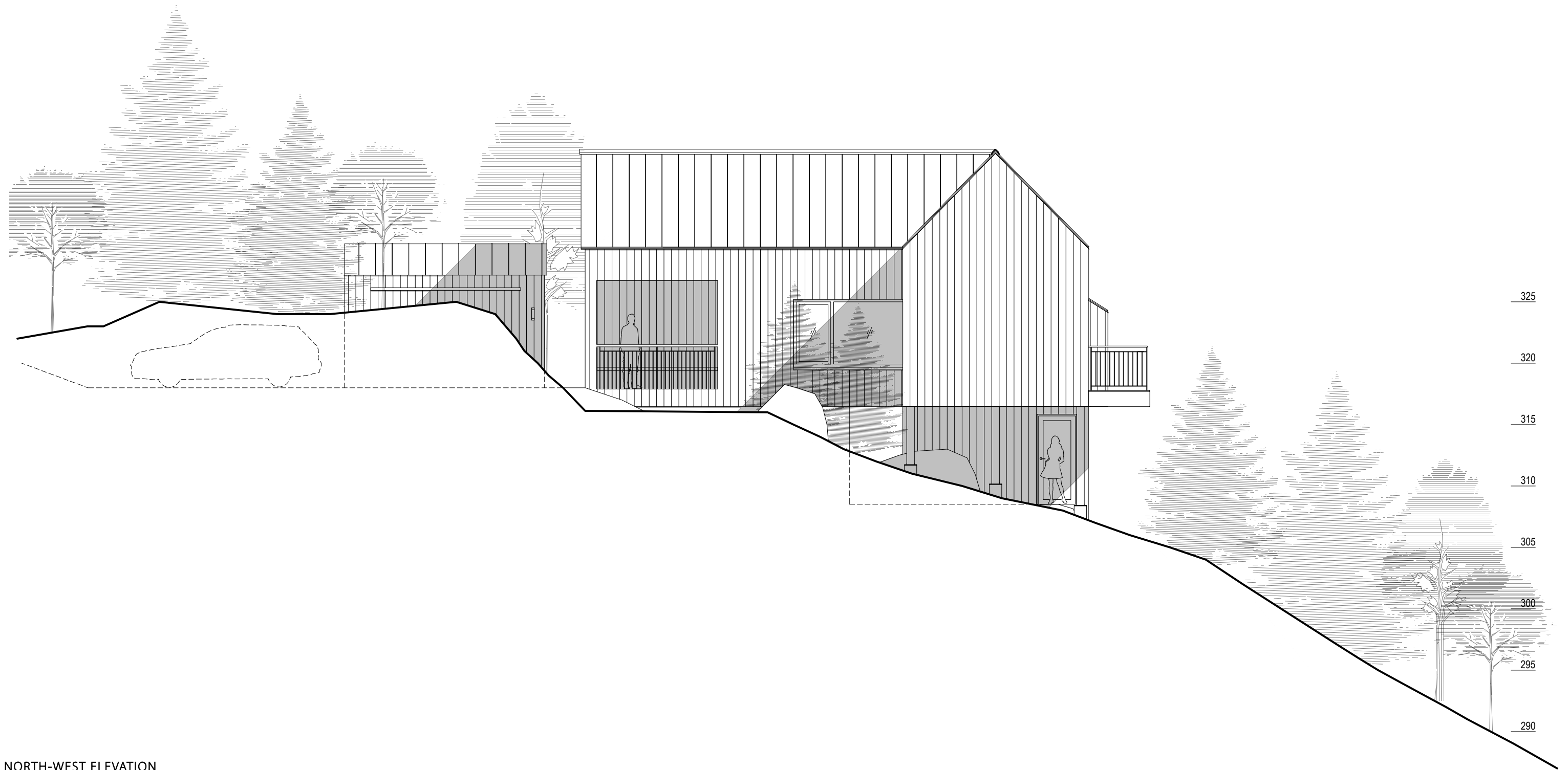
NORTH-WEST ELEVATION CHALET PAPILLON
