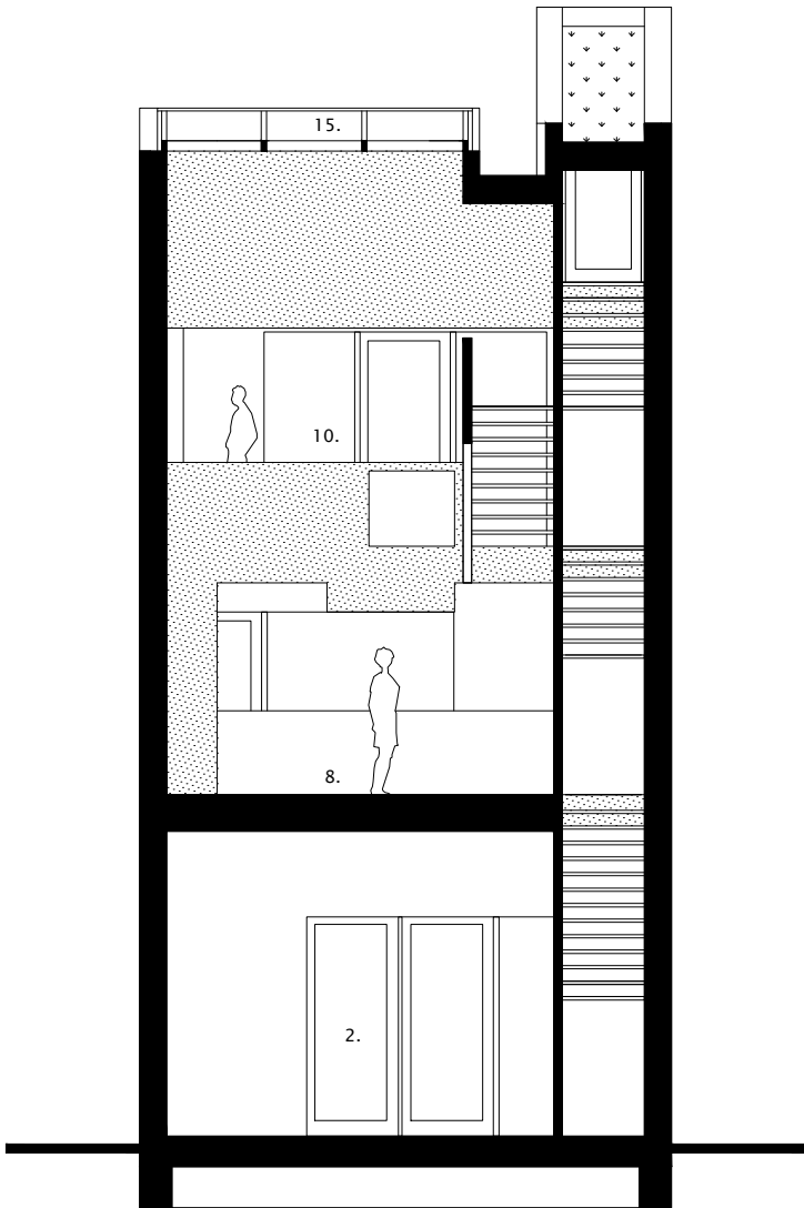
cross section width
