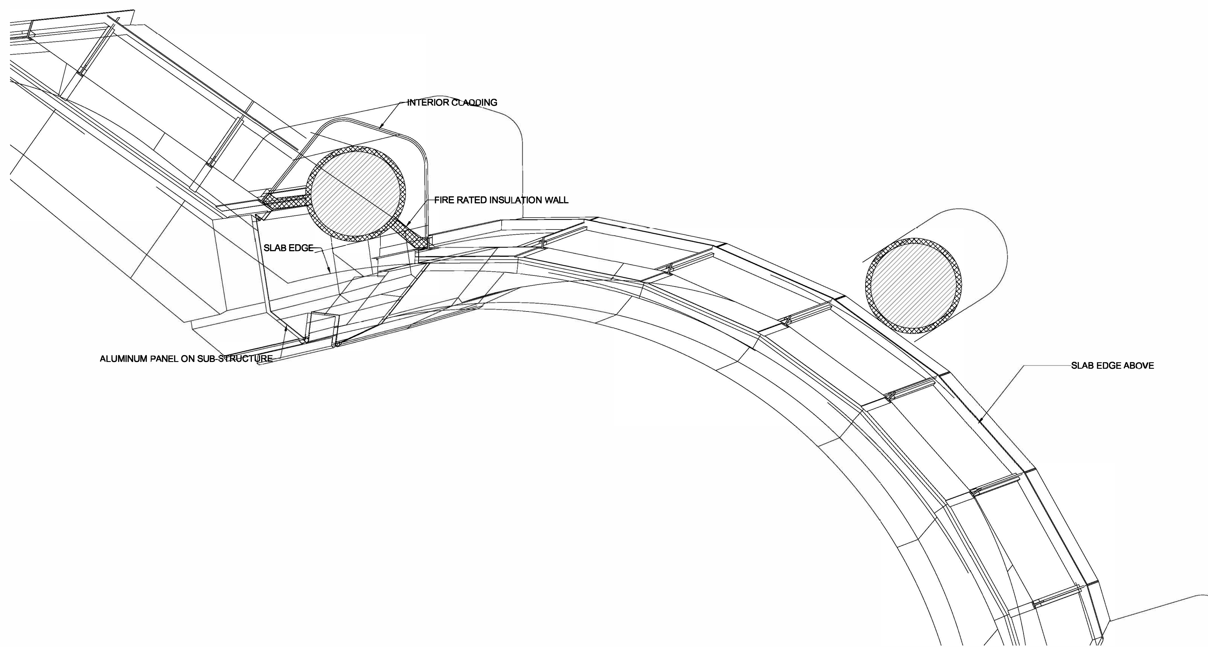
FS3 - ELEVATION, PLAN & SECTION
