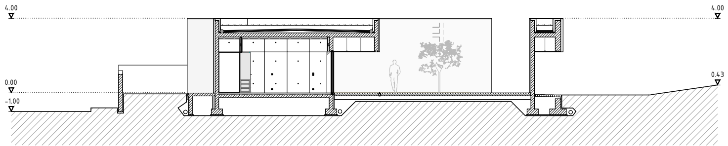
TRANSVERSAL SECTION 02
