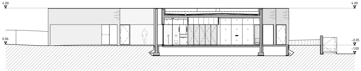
TRANSVERSAL SECTION 01
