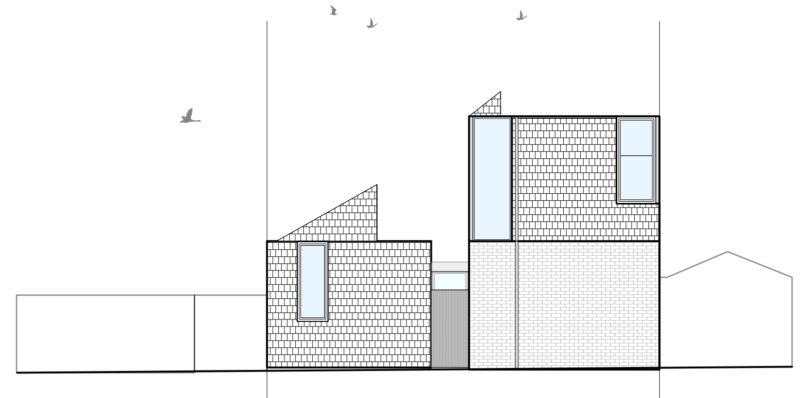
Elevation South
