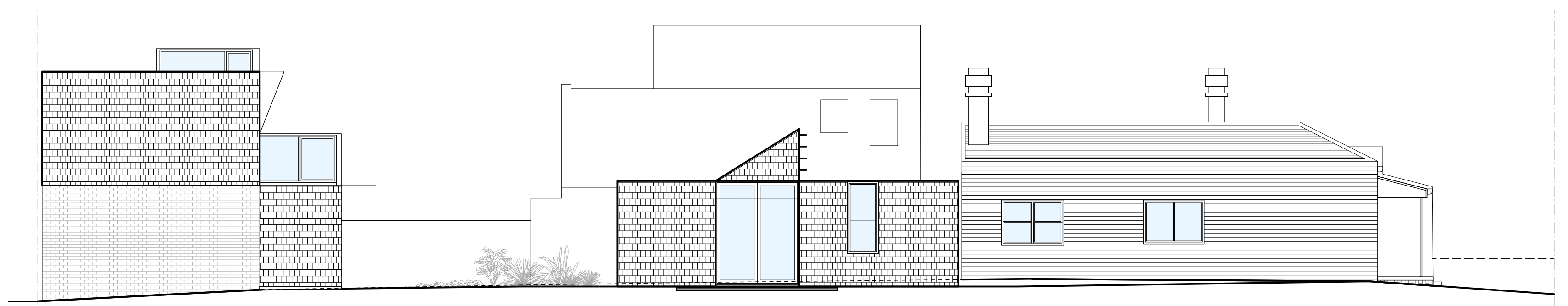
Elevation East
