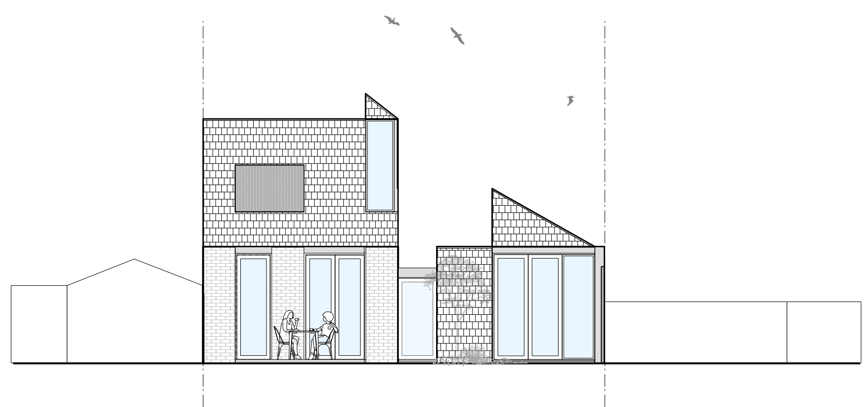
Elevation North
