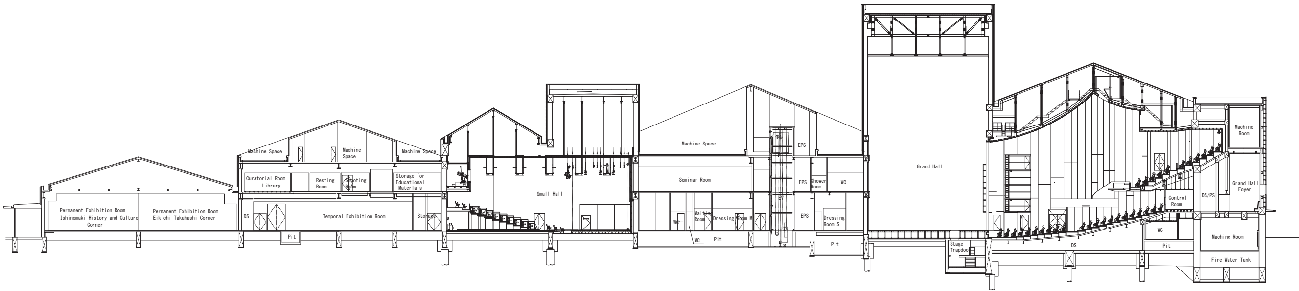
Section B-B
