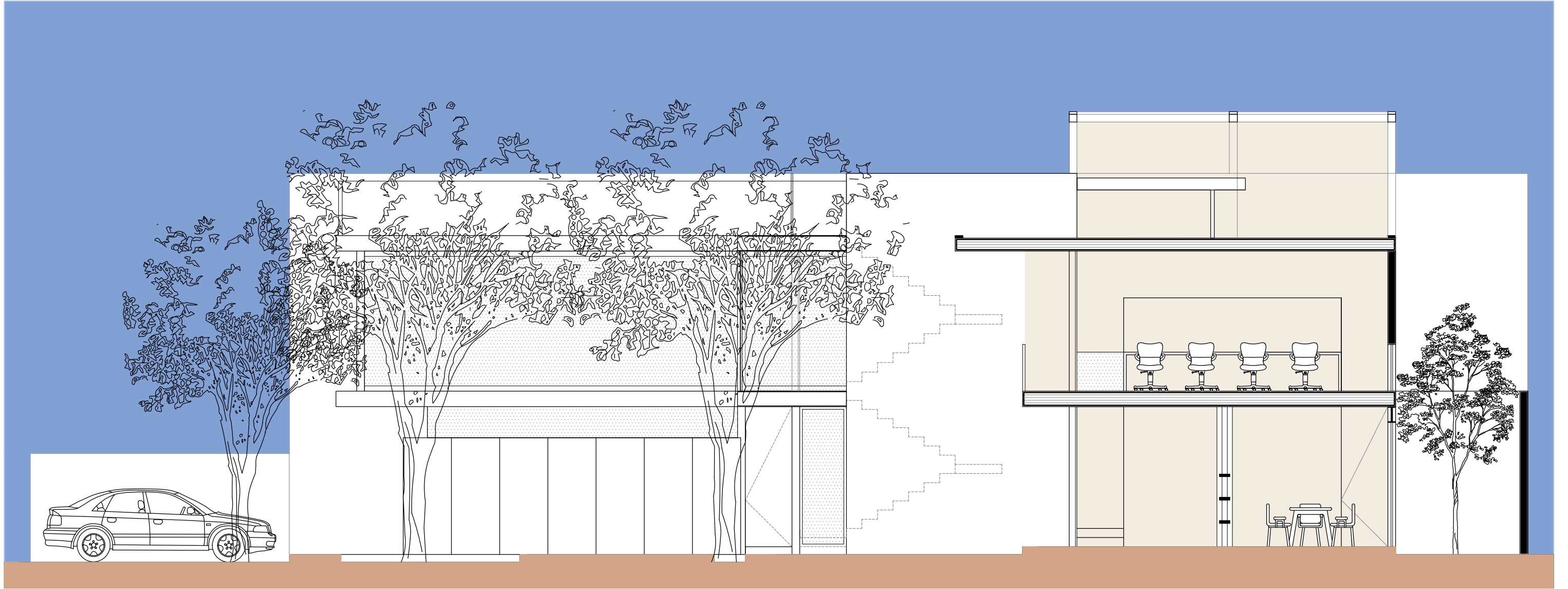
SECTION C-C'
