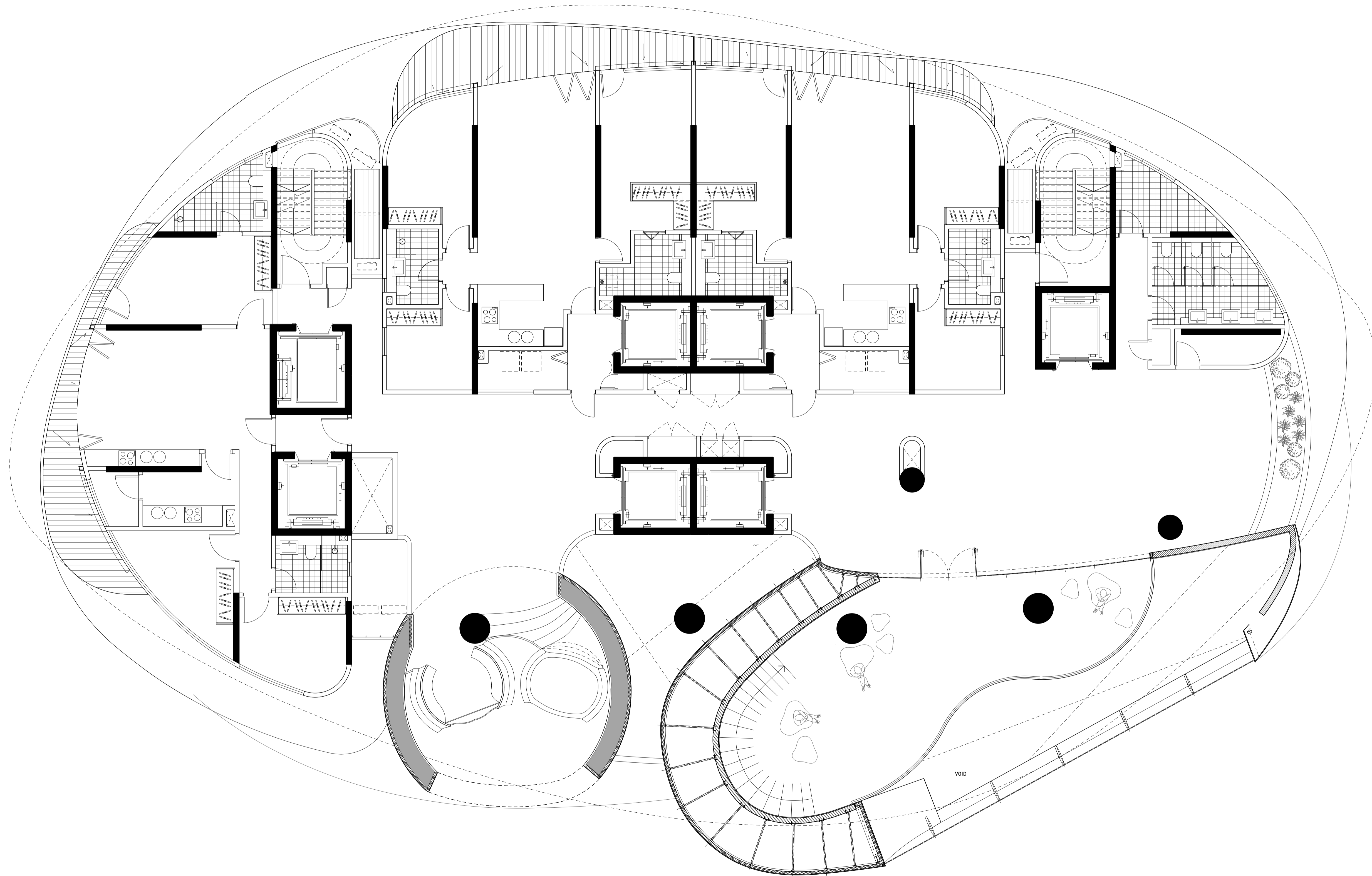
01 TOWER B RESIDENTIAL PLAN AT LEVEL 37 1:75
