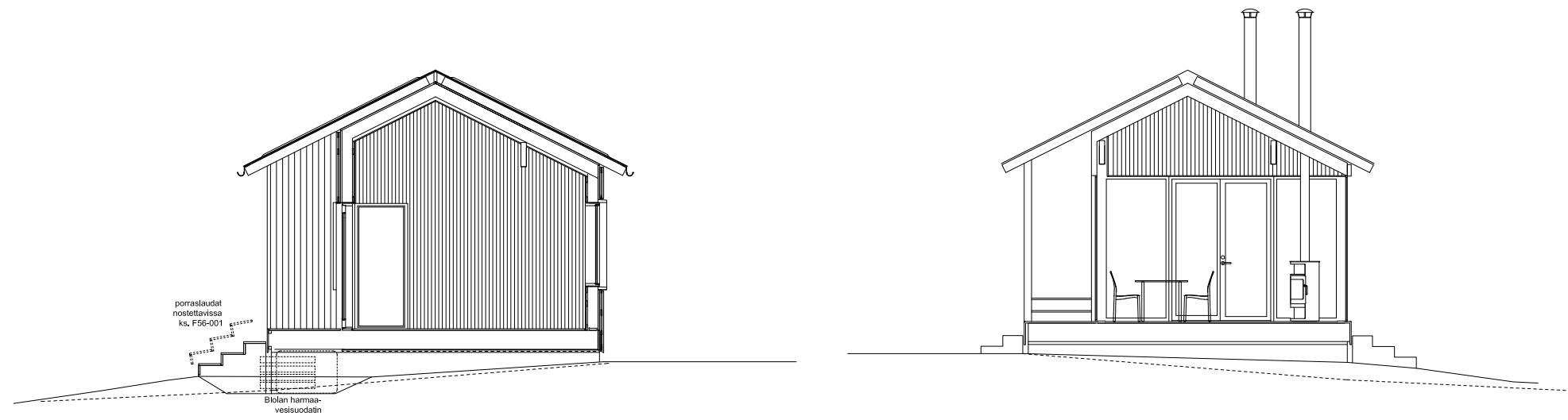
SECTIONS 1:100
