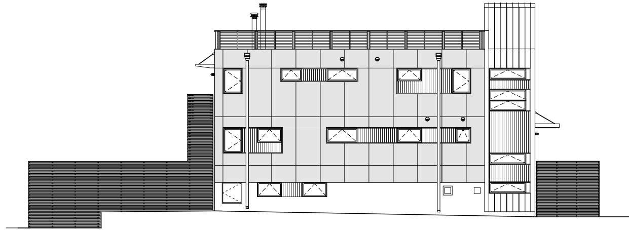
NORTH ELEVATION
