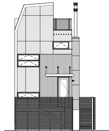
WEST ELEVATION
