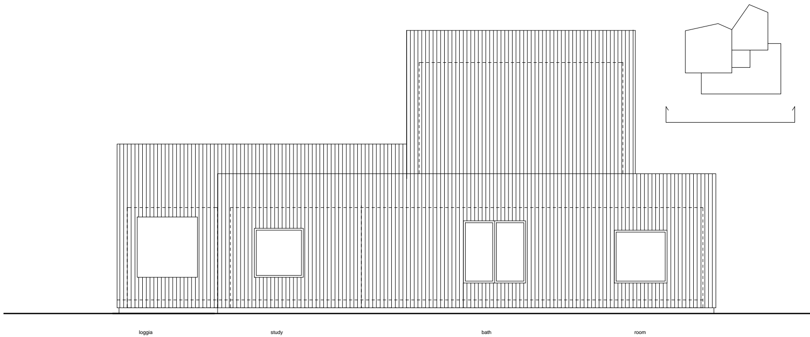
Facade/east 1 : 50
