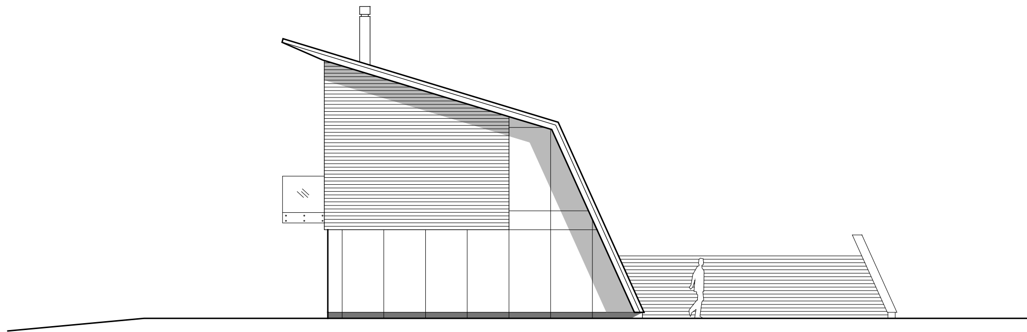
EAST ELEVATION
