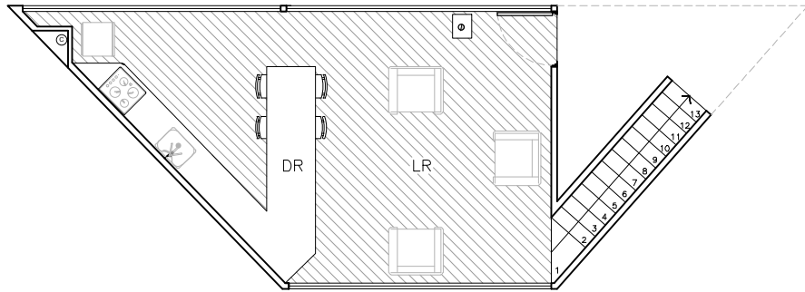
1ST FLOOR PLAN 0 50 100
