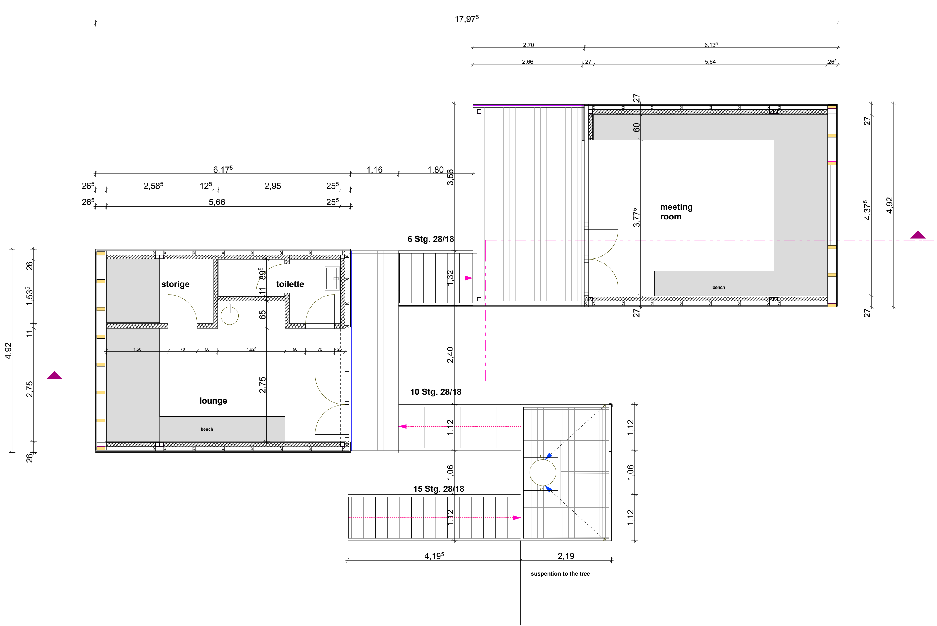
floor plan
