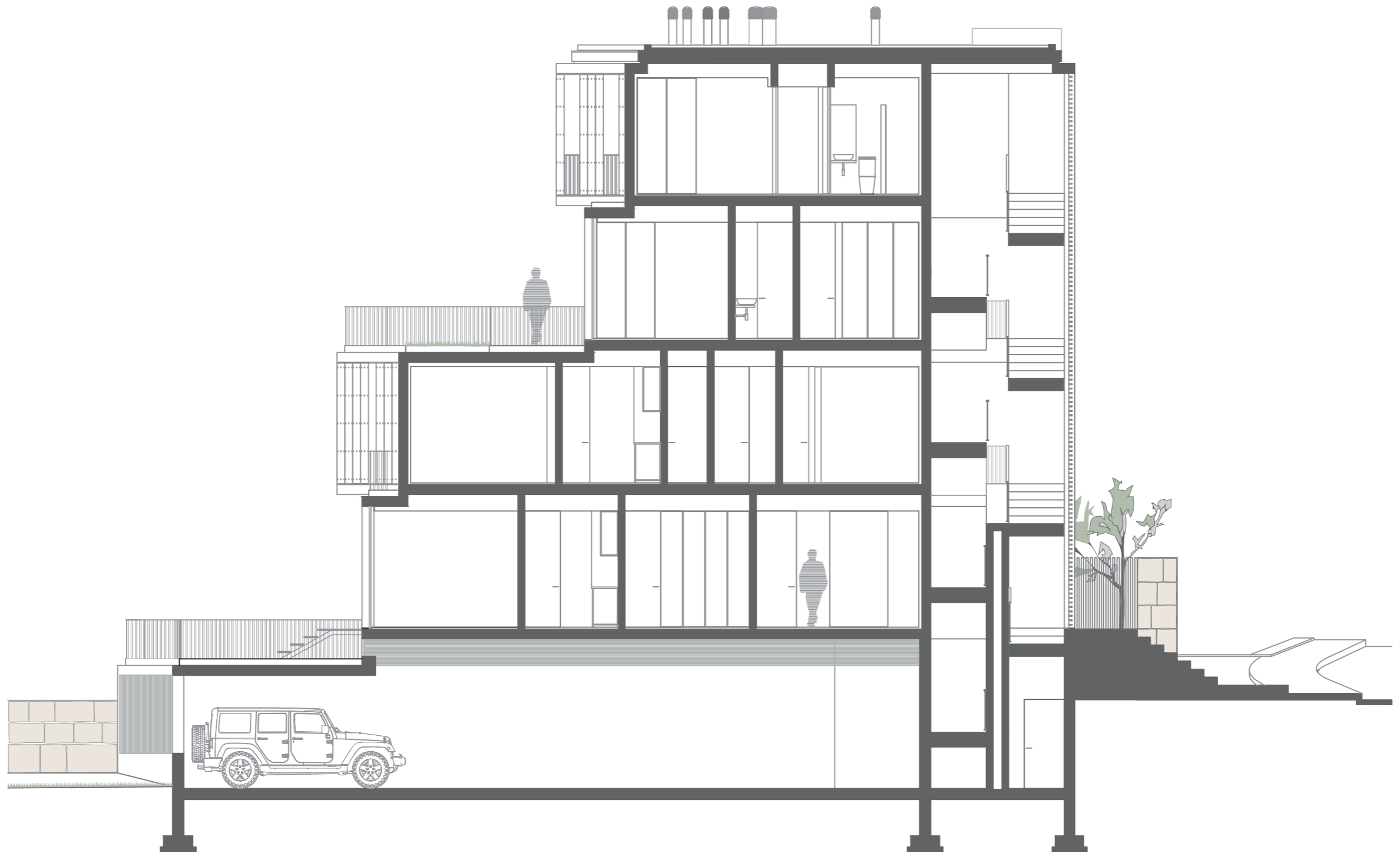
TORRE 261 | SECTION
