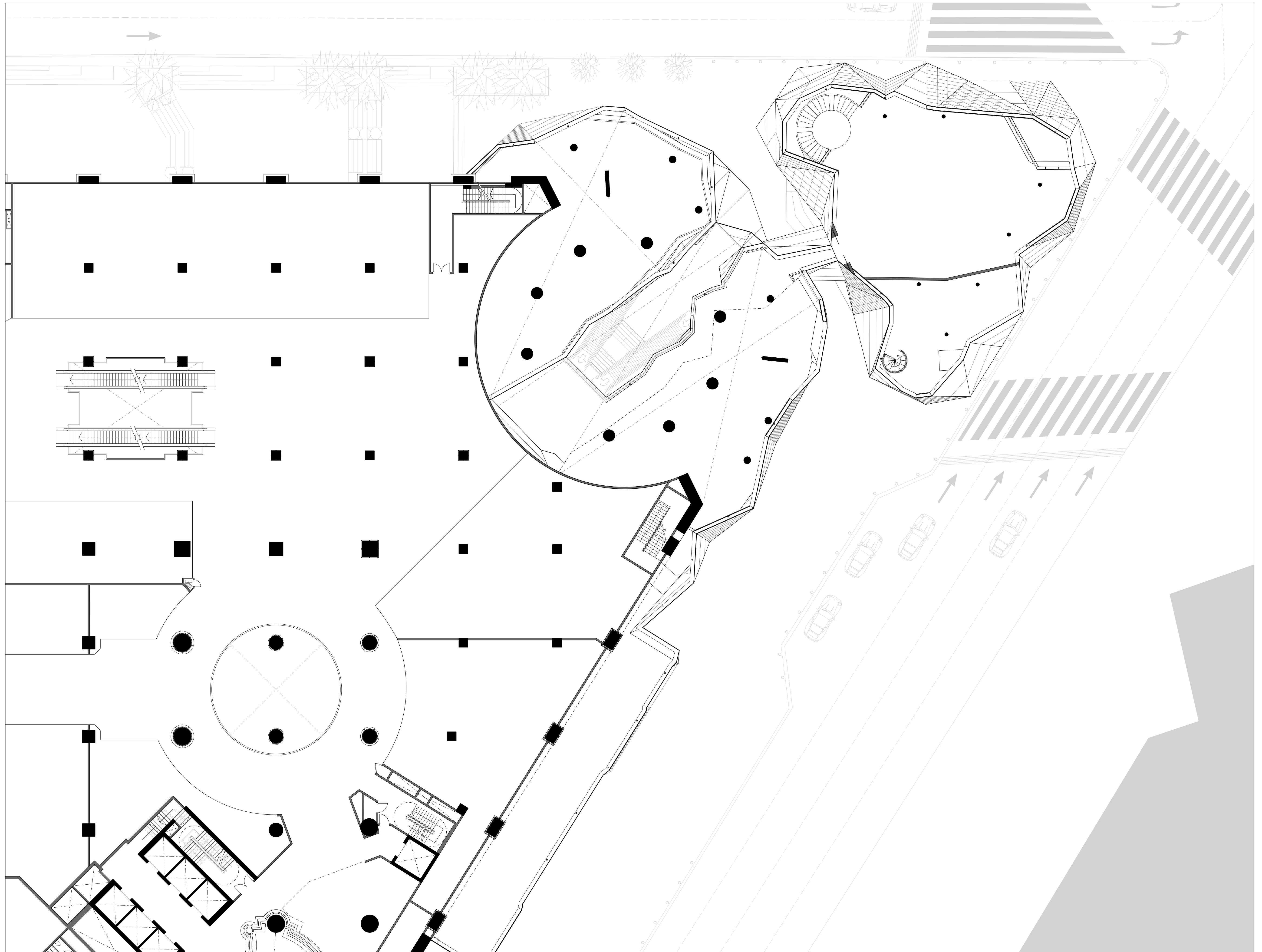
1 GENERAL ARRANGEMENT / PLAN LEVEL 5 GA/p103 SCALE 1:150
