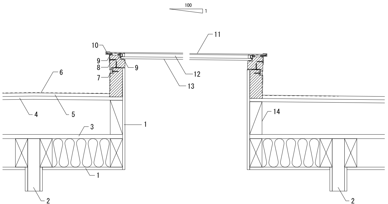
top light detailed section 1/8
