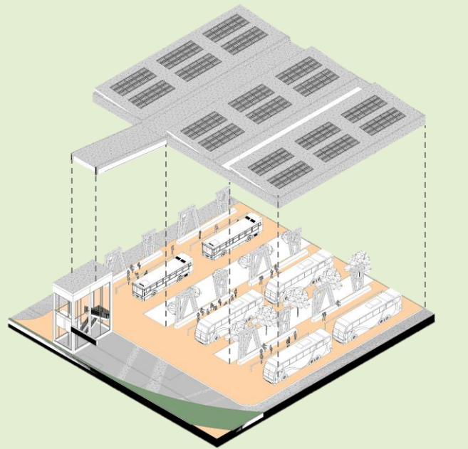
Perspective
