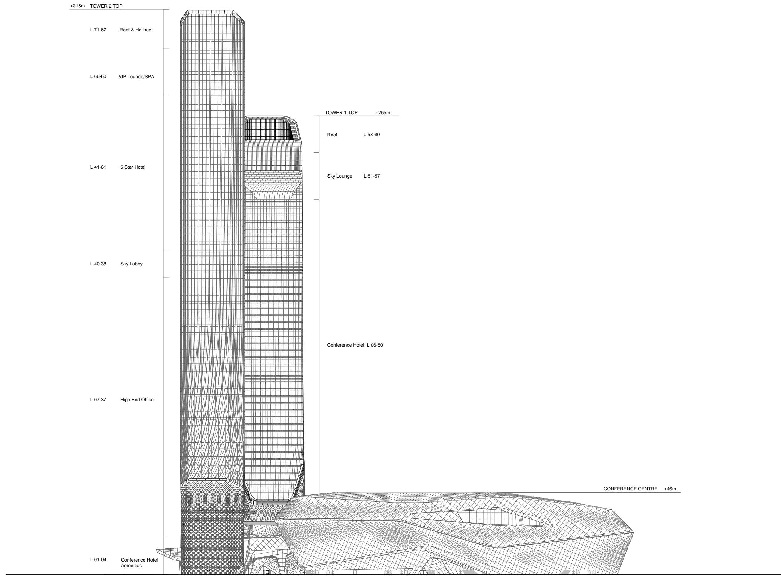
EAST ELEVATION Nanjing International Youth Cultural Centre 1 5 10 20 50
