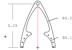
Short link Laser cutting, Steel 3mm
