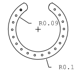
Ring Laser cutting, Steel 3mm
