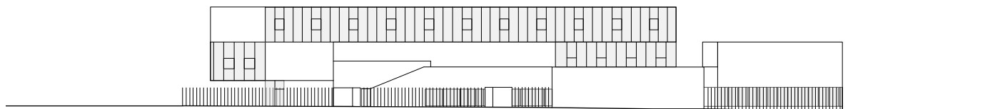
north elevation
