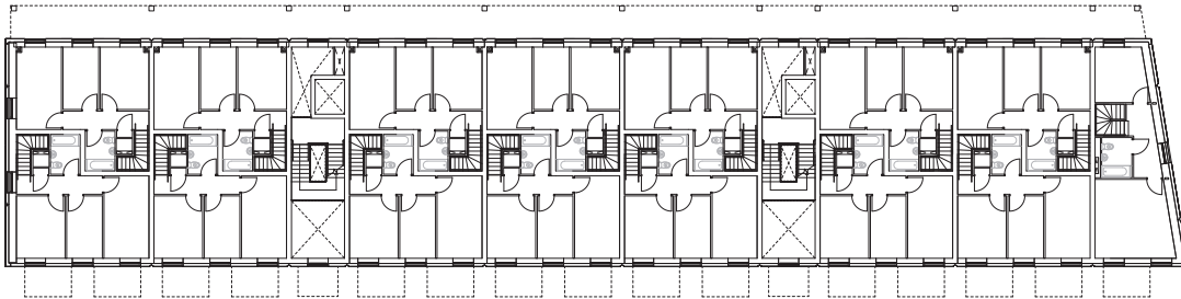
Third floor - Block B1
