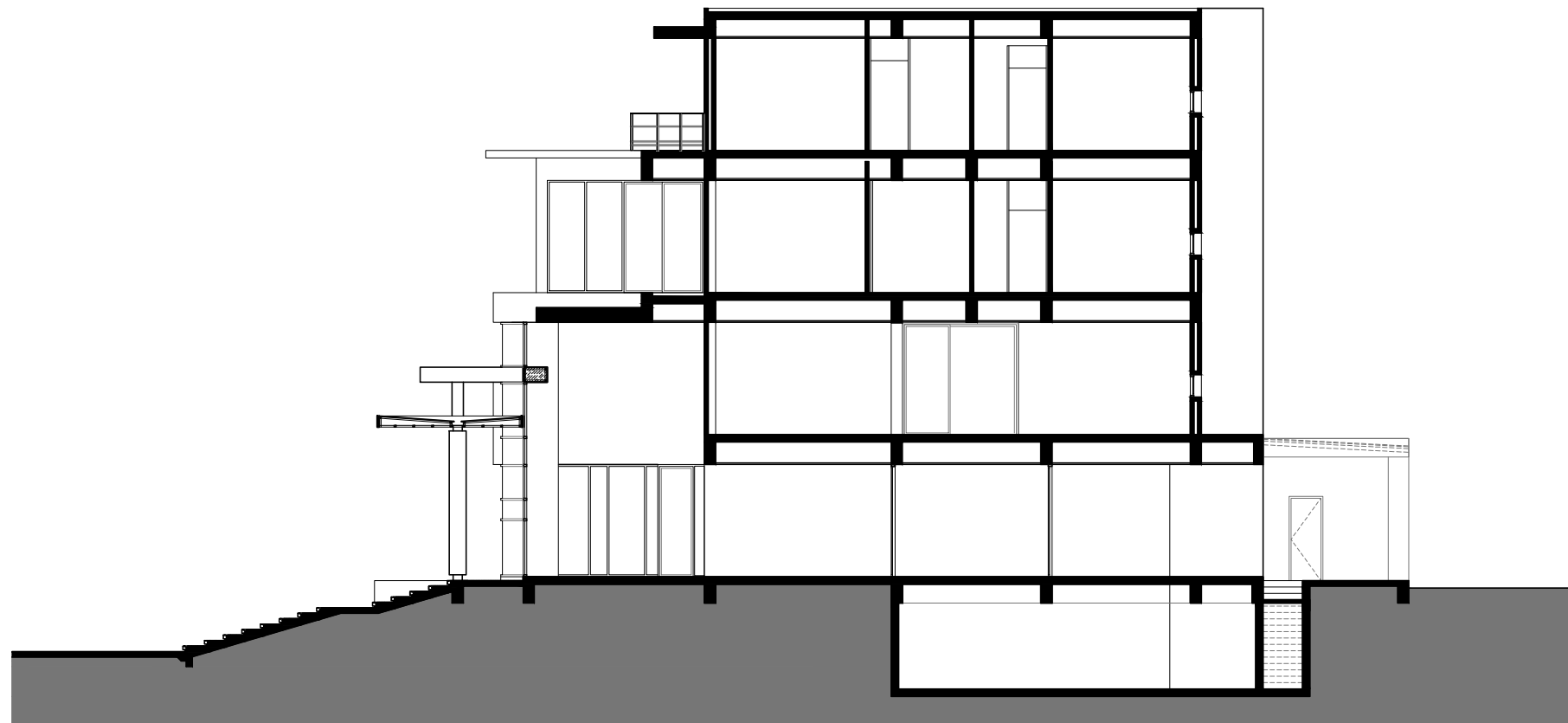
C-C SECTION
