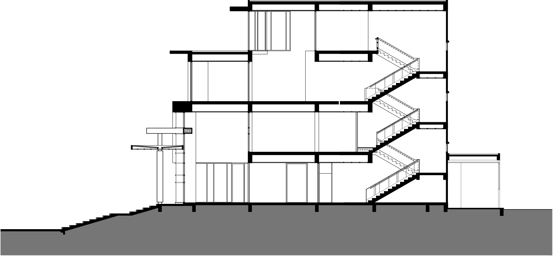
B-B SECTION
