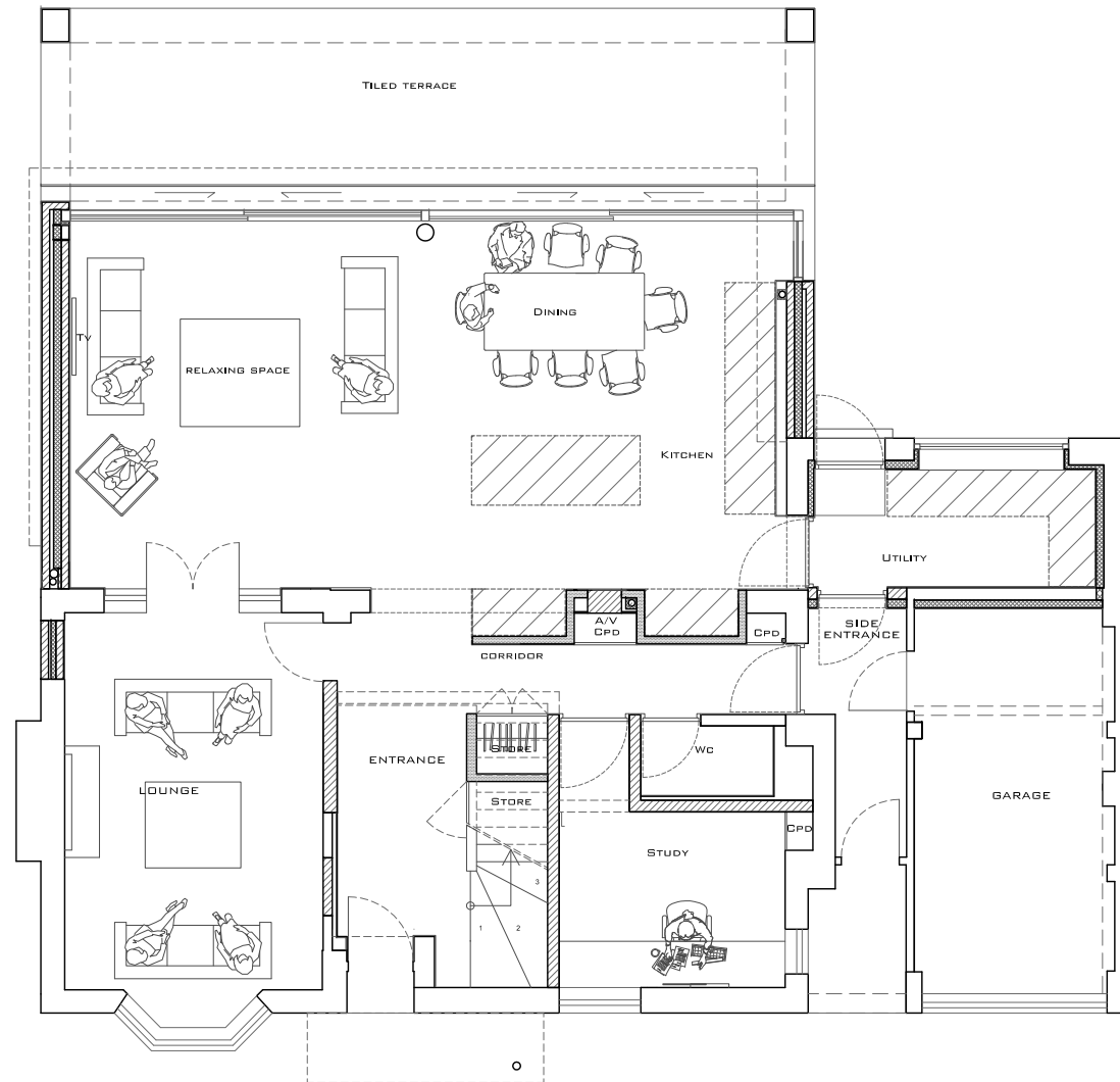
GROUND PLAN
