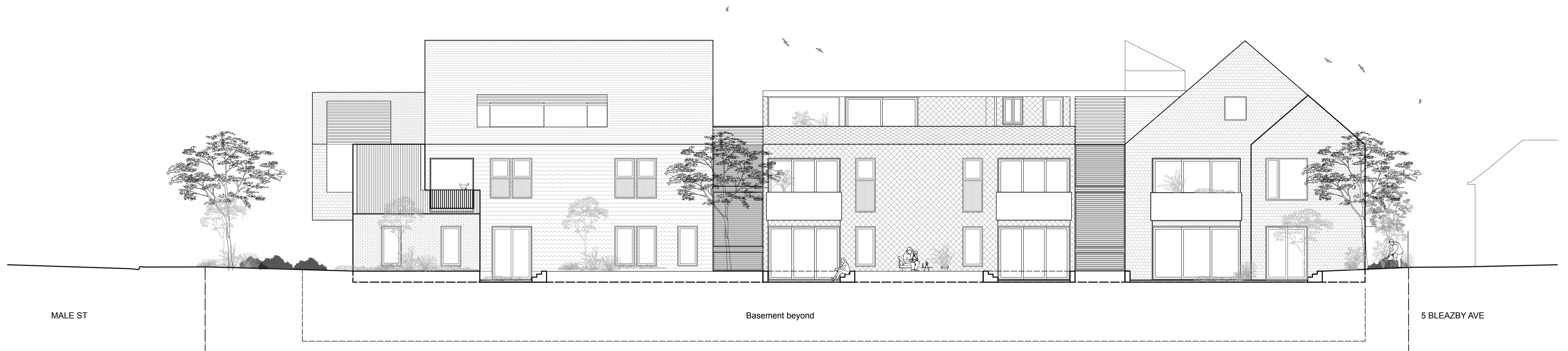
Northern Elevation
