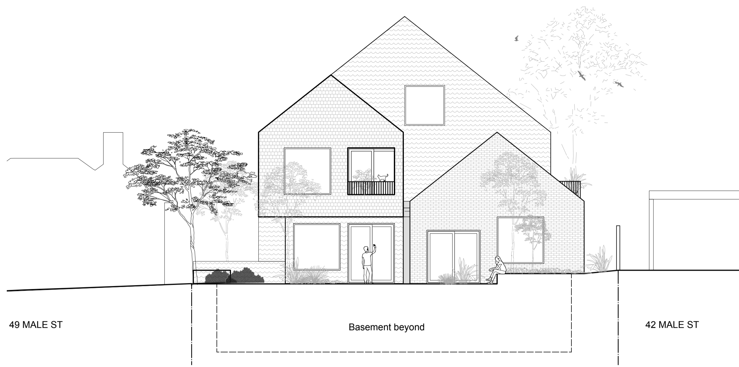
Eastern(Male Street) Elevation
