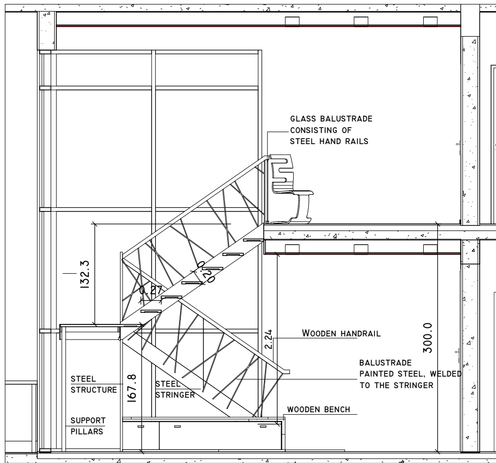
SECTION CC _ SCALE 1:50
