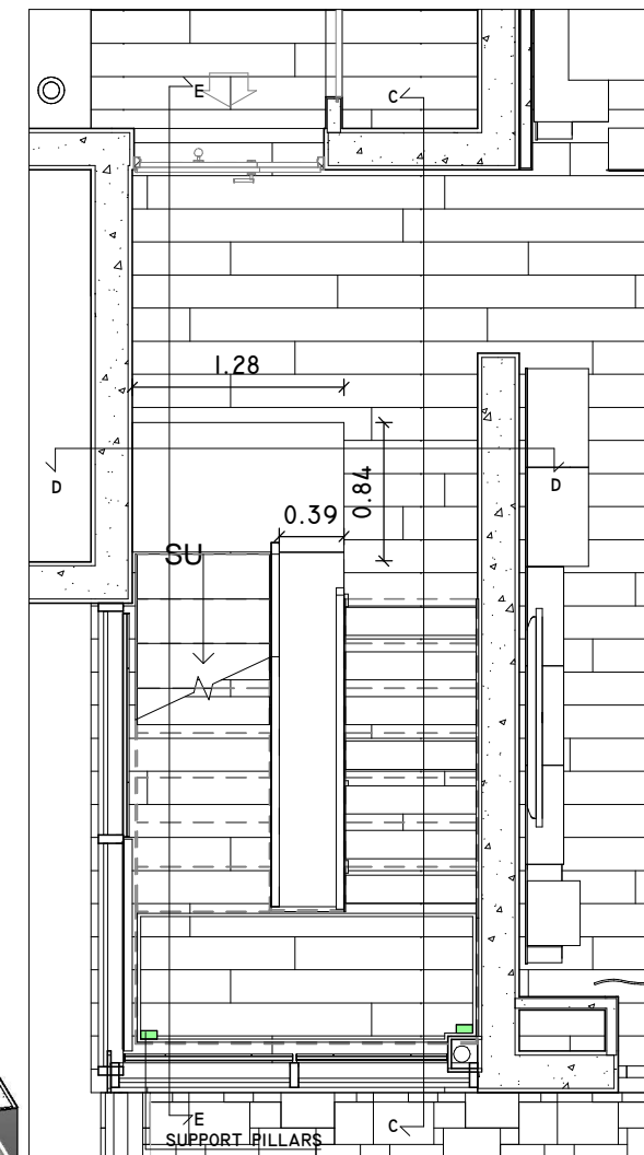
STAIR DETAIL _ SCALE 1:50
