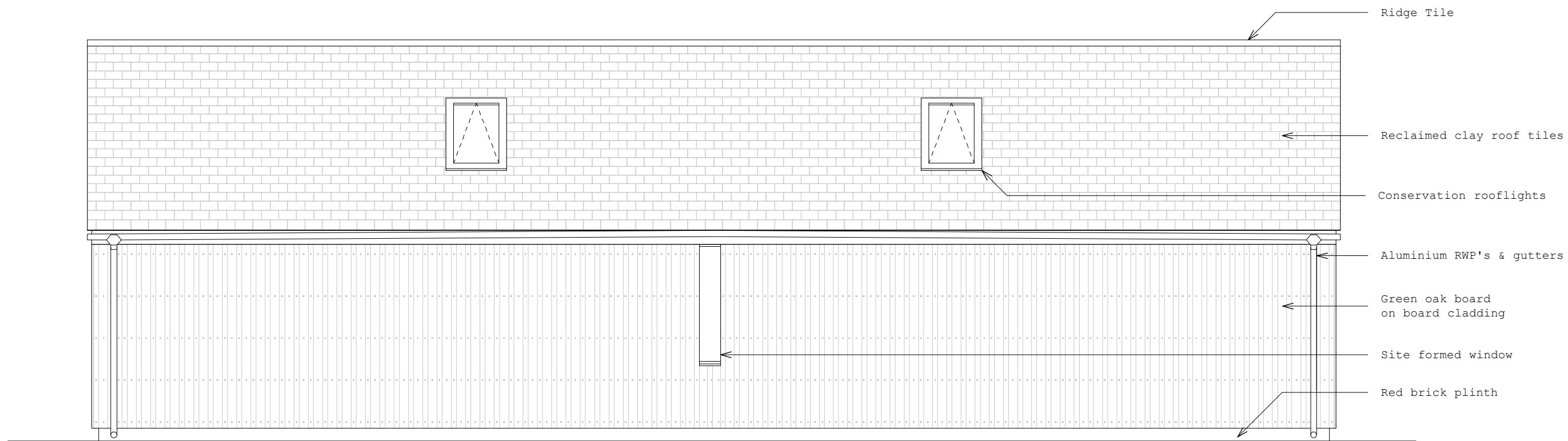
SOUTH WEST ELEVATION 1:50 @ A3
