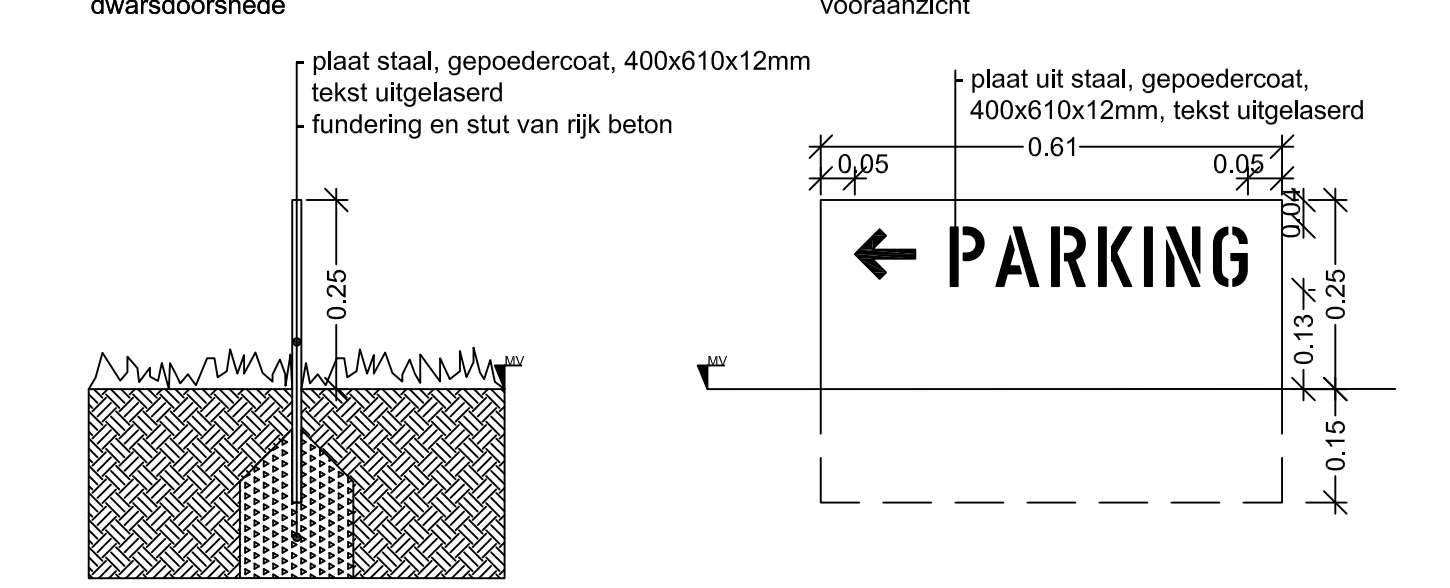
Infopaneel A1 1:10
