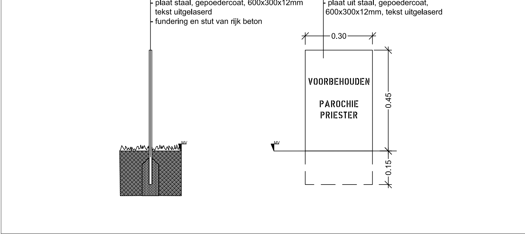
infopaneel A3 1:10
