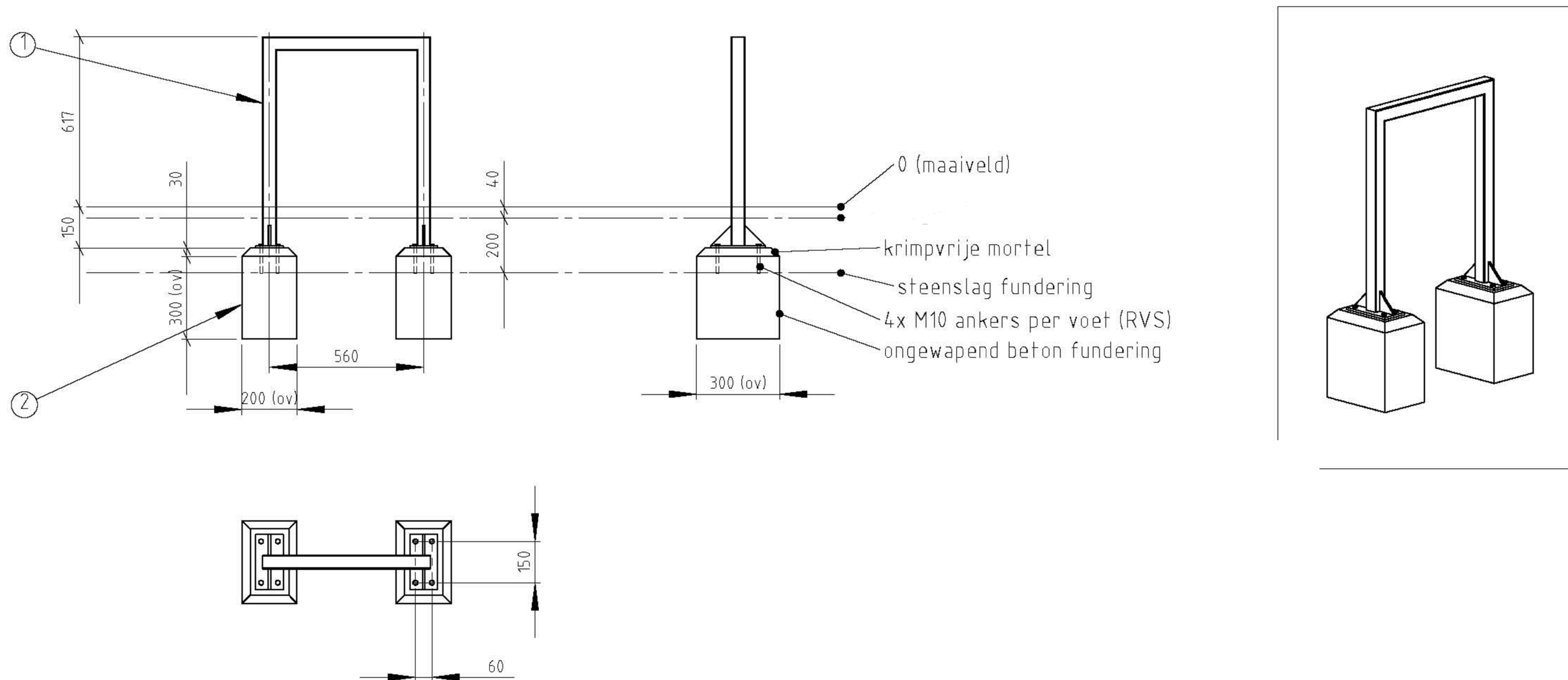
fletsframe 1:10
