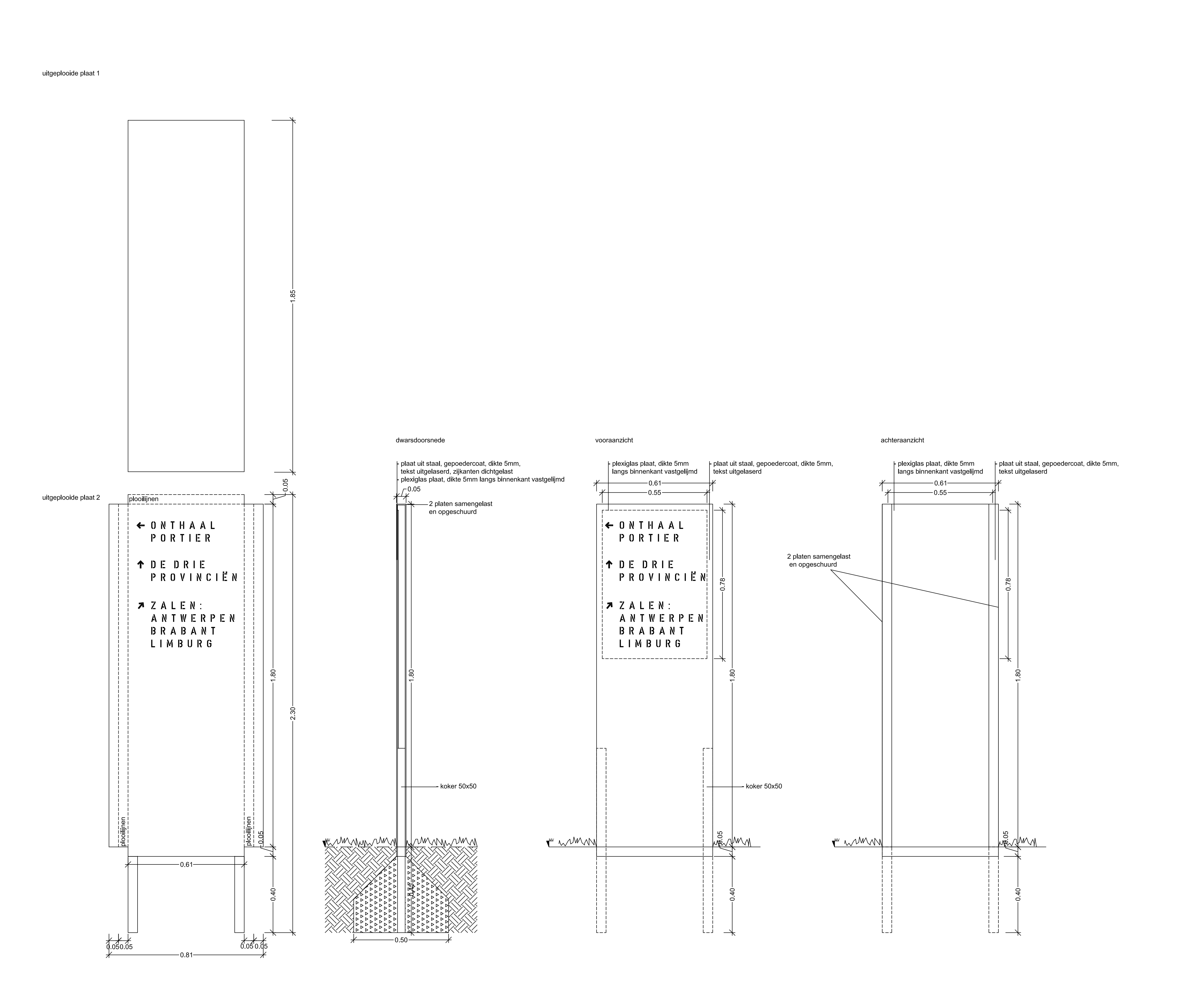
Infopaneel A1 1:10
