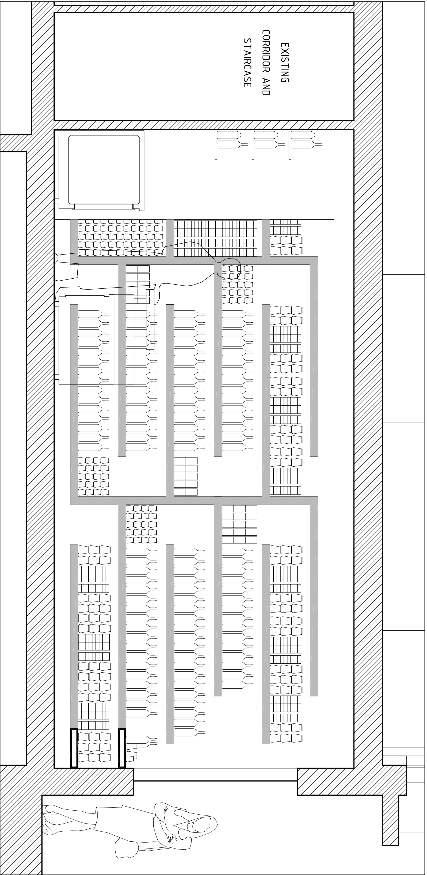
CROSS SECTION - scale 1:25 detail of shelves
