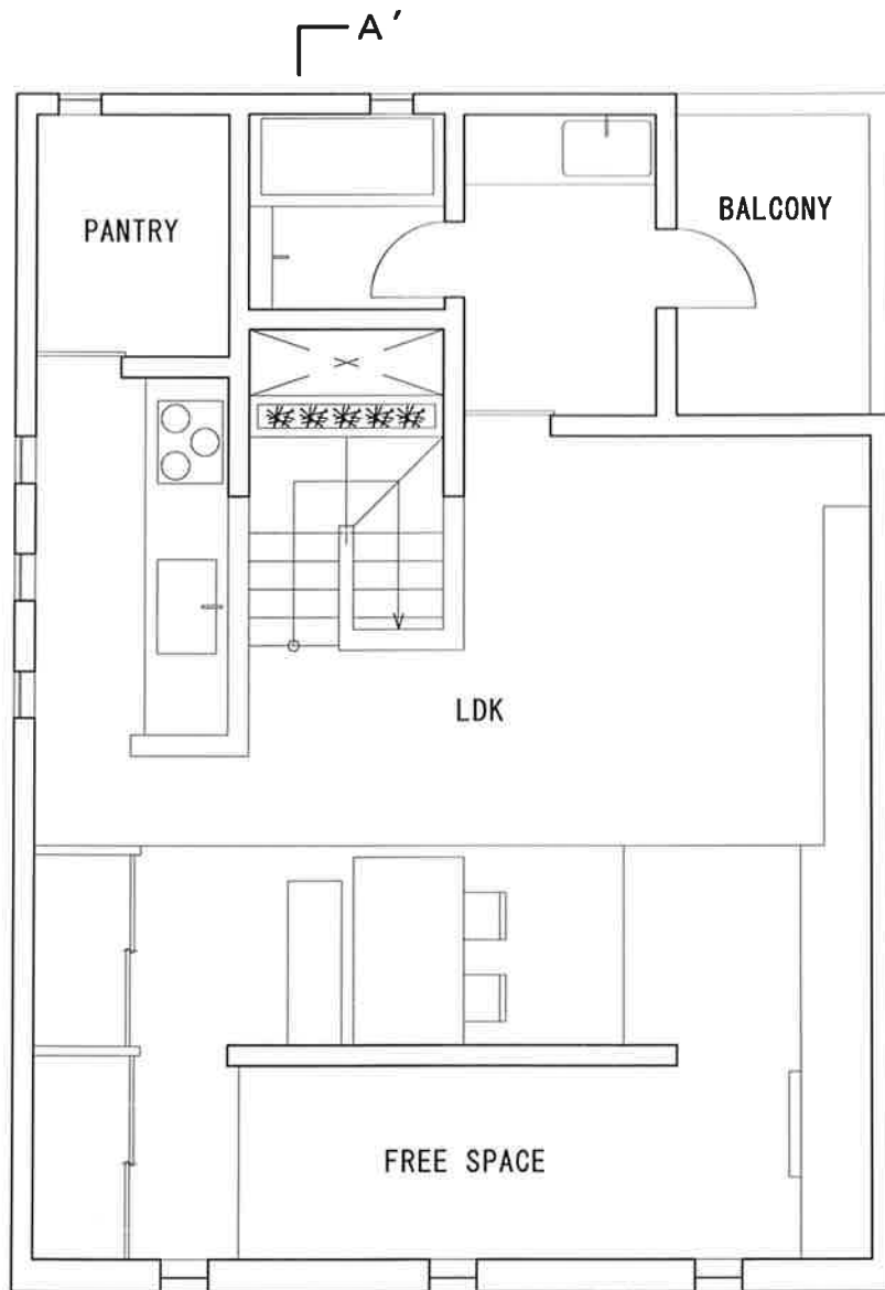
A 2F PLAN
