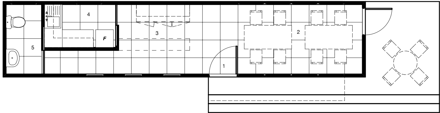
Floor Plan 1:75m
