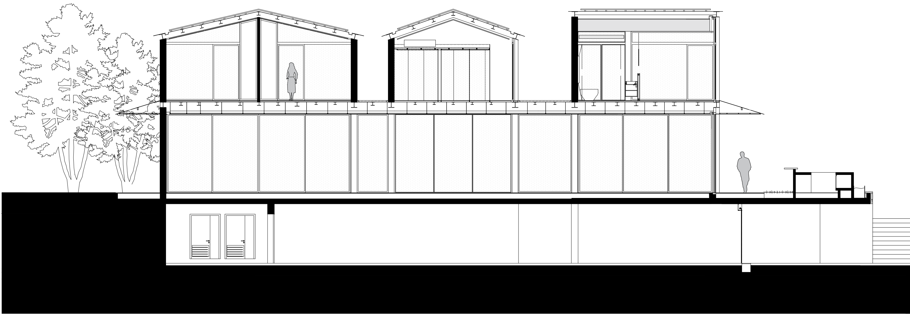
SECTION AA
