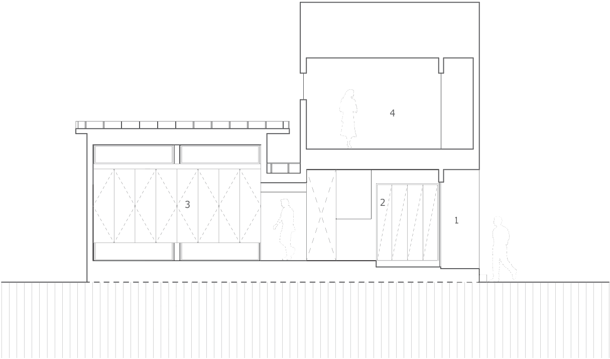
sectional view 1:100
