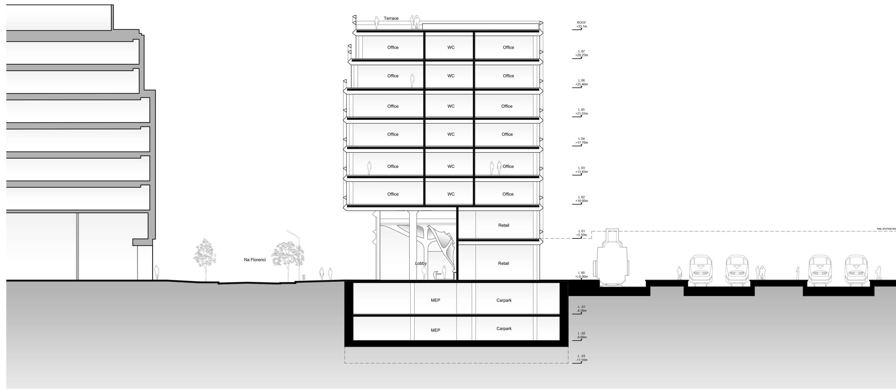
1 SHORT SECTION Scale: 1/300
