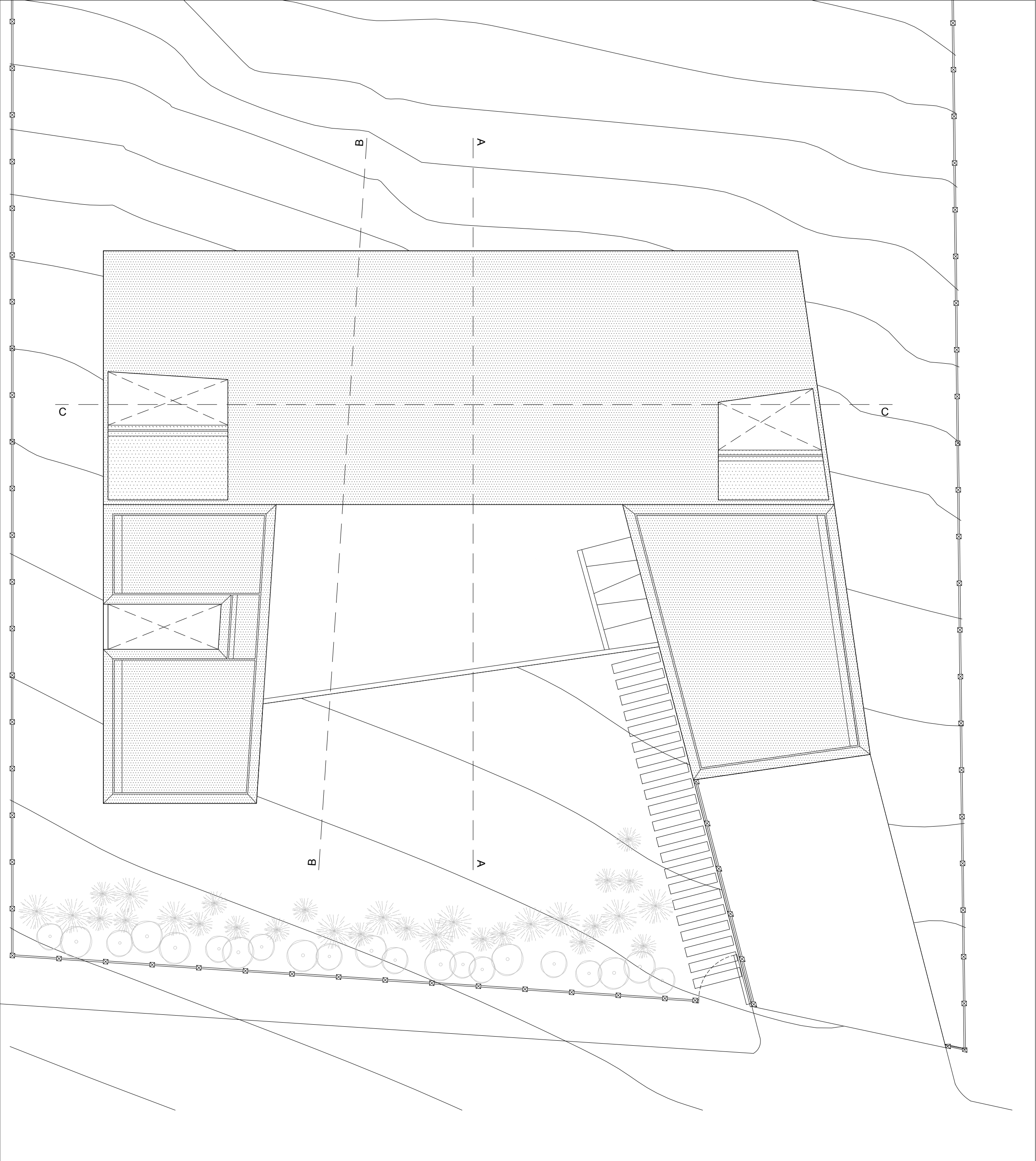
ROOF PLAN
