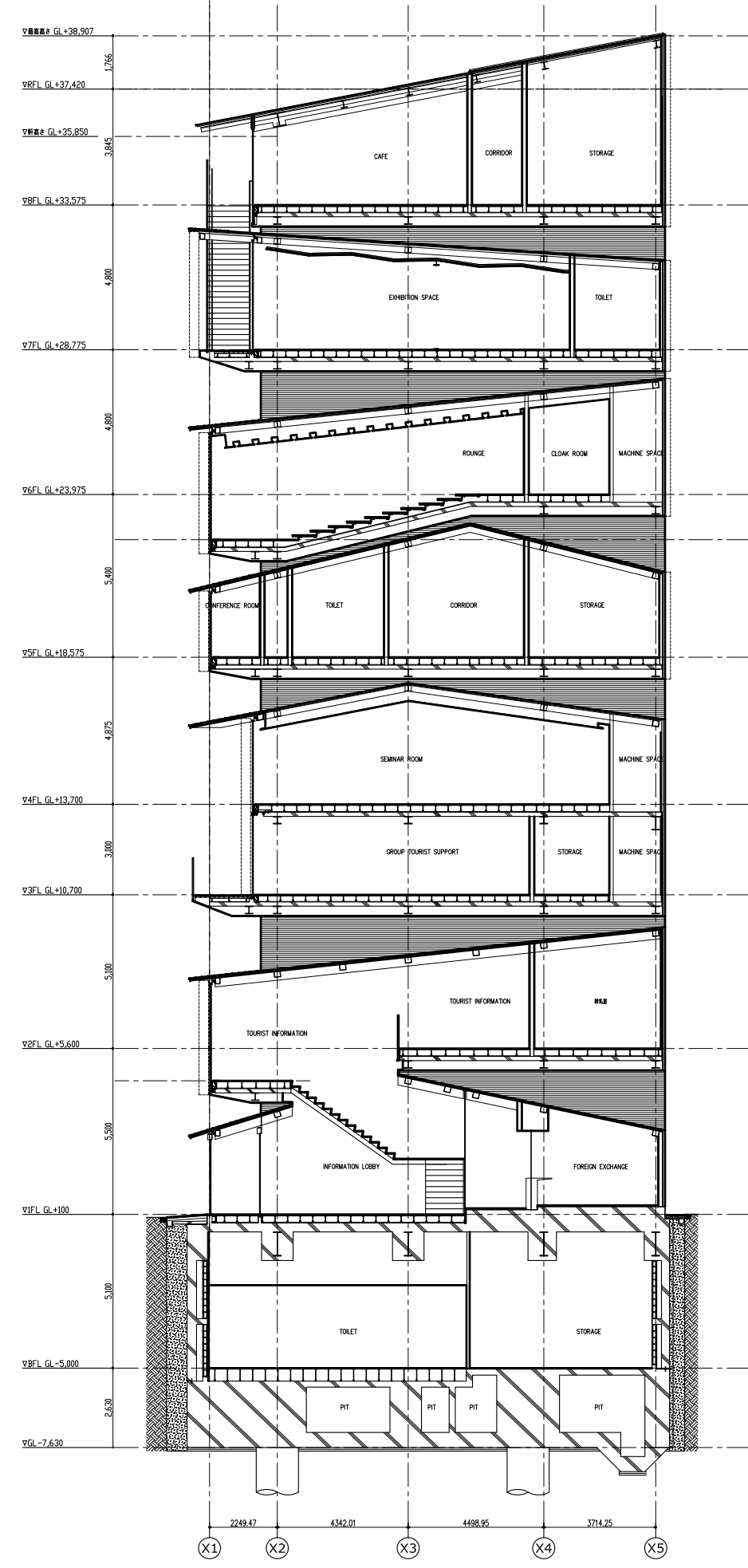
DD' SECTION
