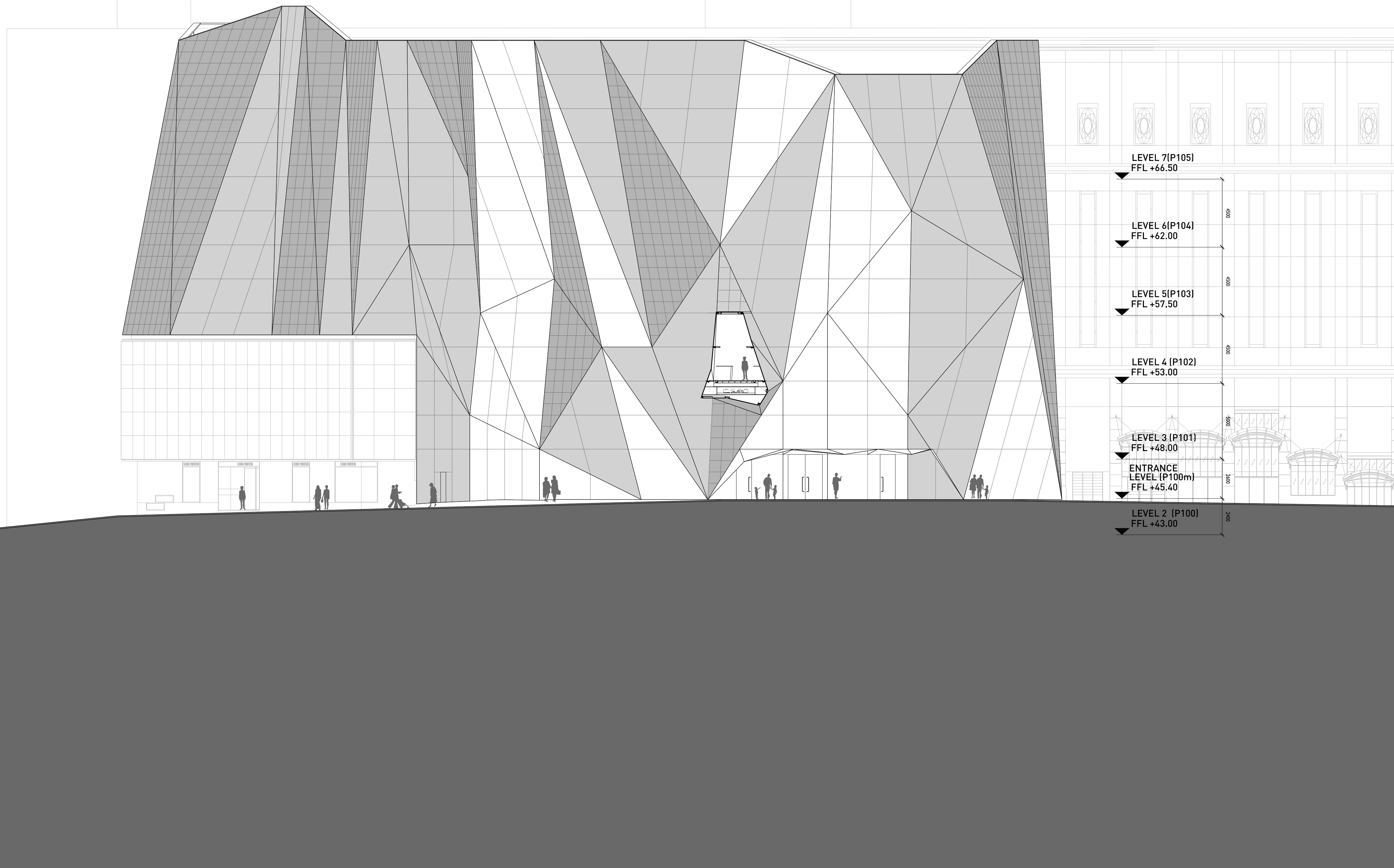
1 ELEVATION AT GALLERY MAIN ENTRANCE GA/e305 SCALE 1:150
