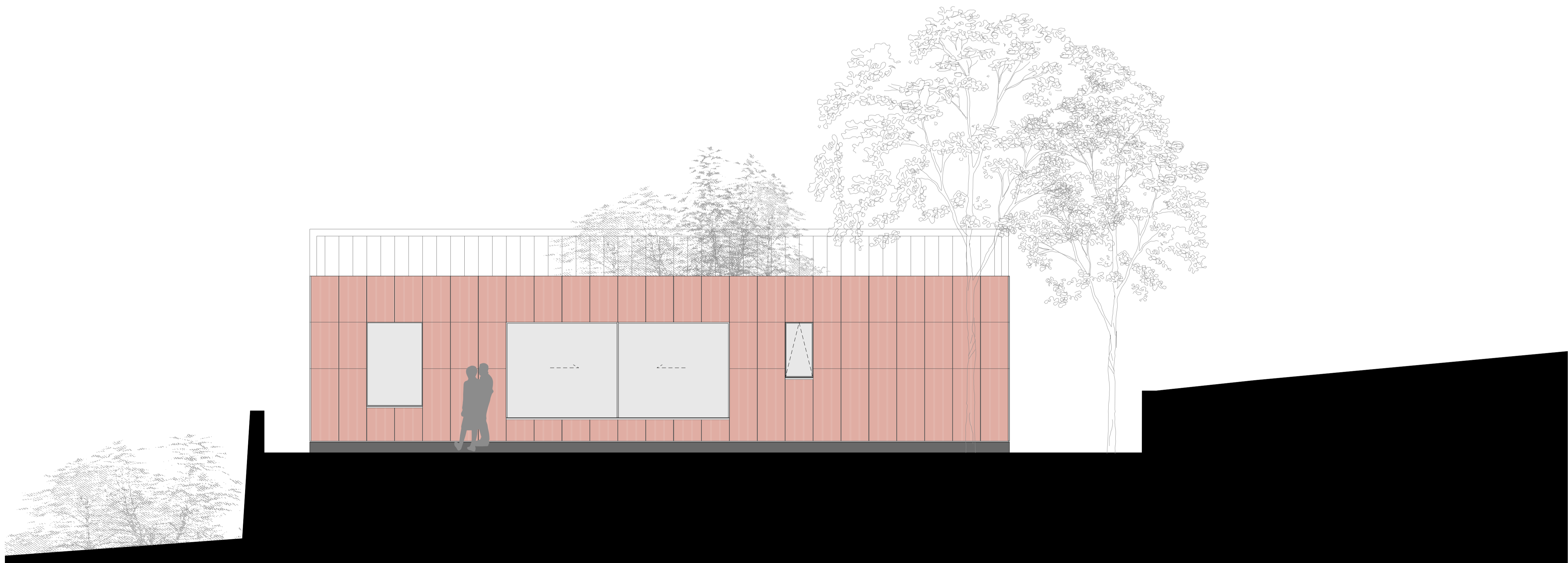
E04 - West Elevation
