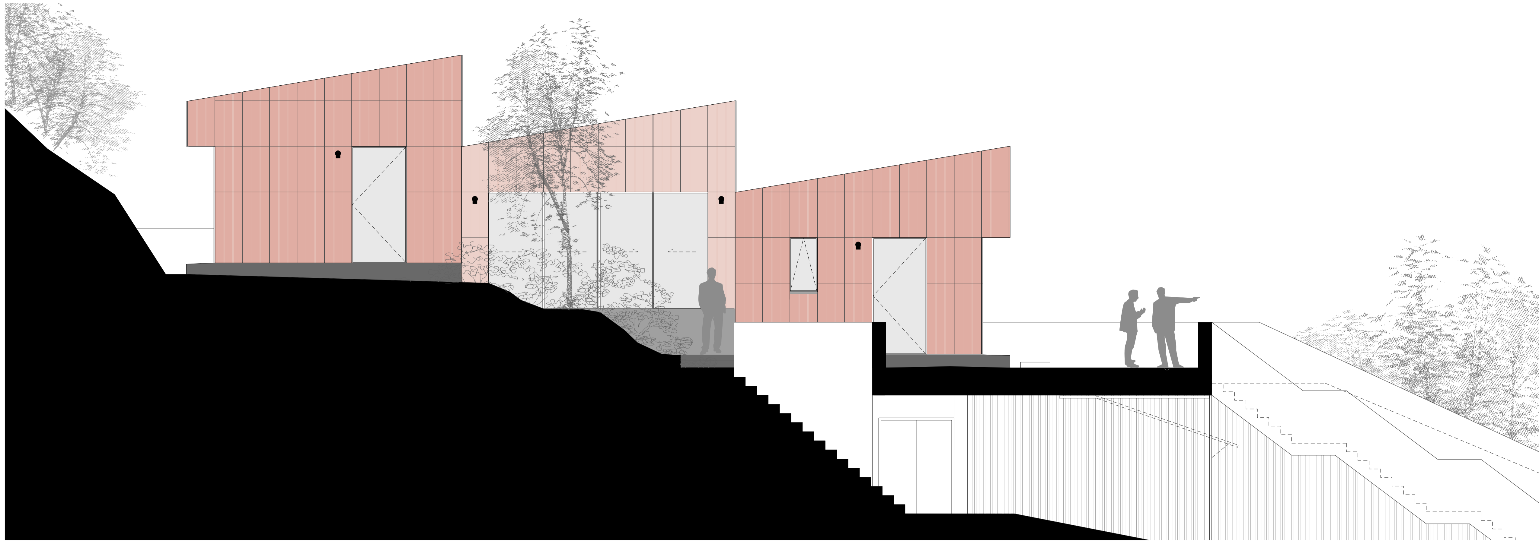
E03 - South Elevation
