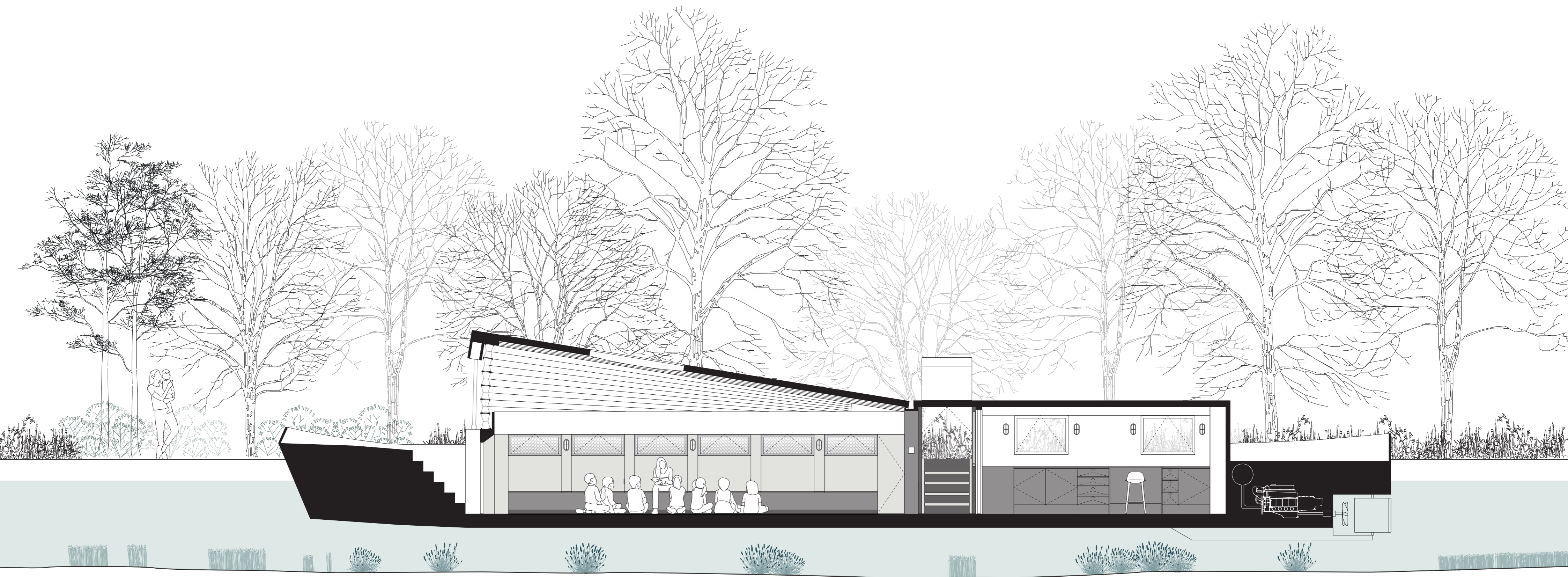
THE FLOATING CHURCH LONG SECTION_ROOF OPEN 1:25@A2
