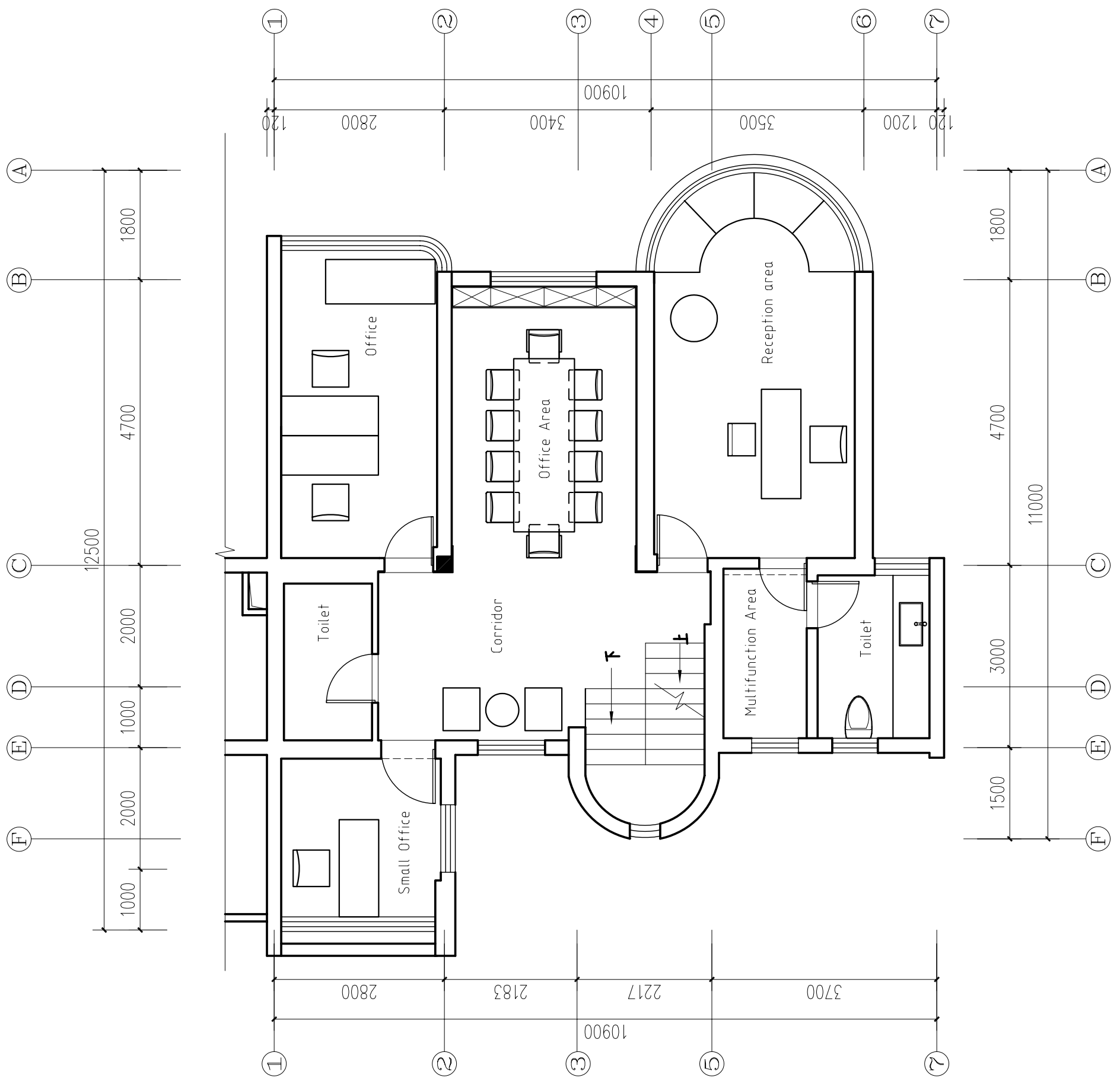
The 2 floor plan A3 SCALE 1:75
