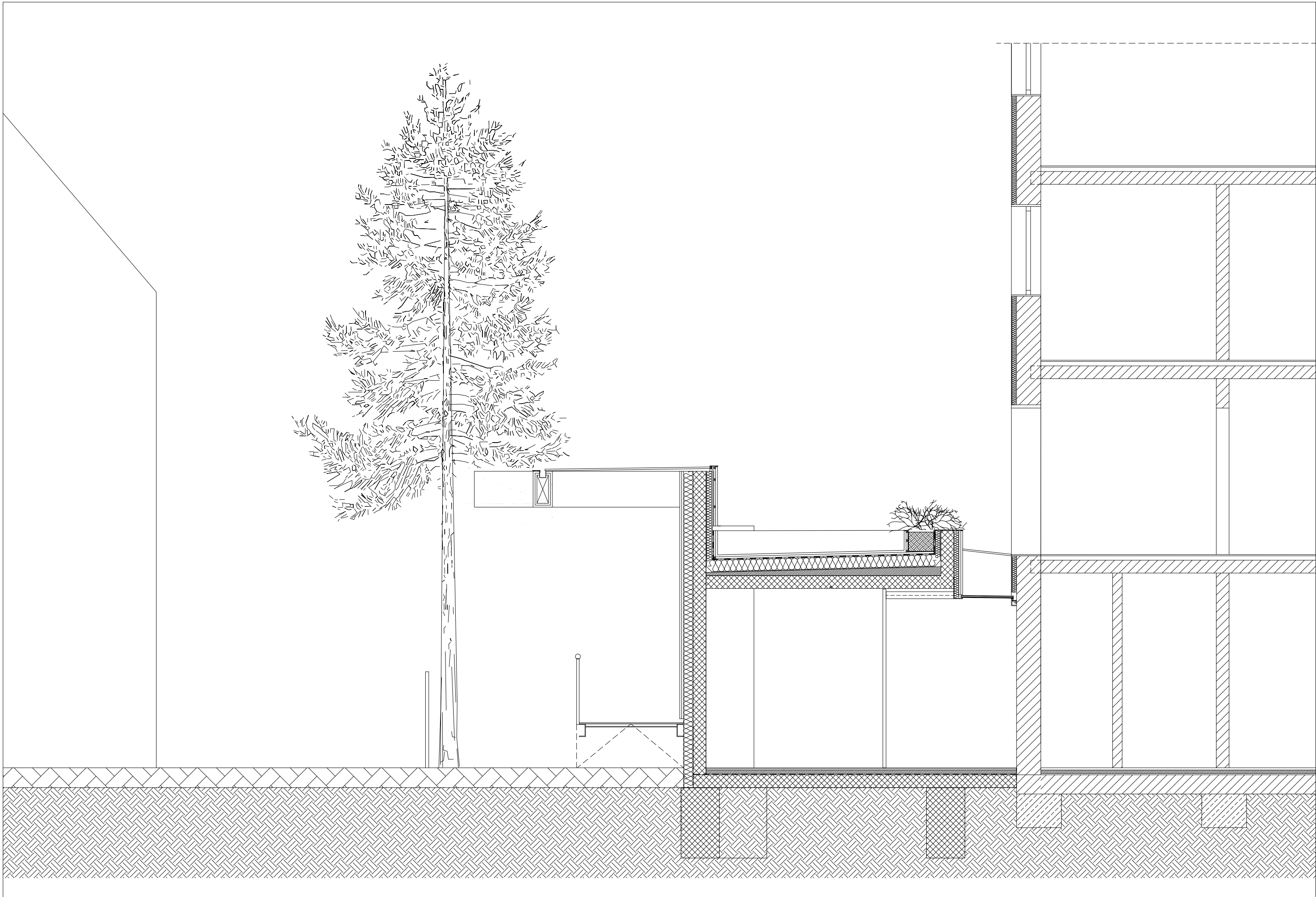
TRANSVERSE SECTION 0 1 2 (1)
