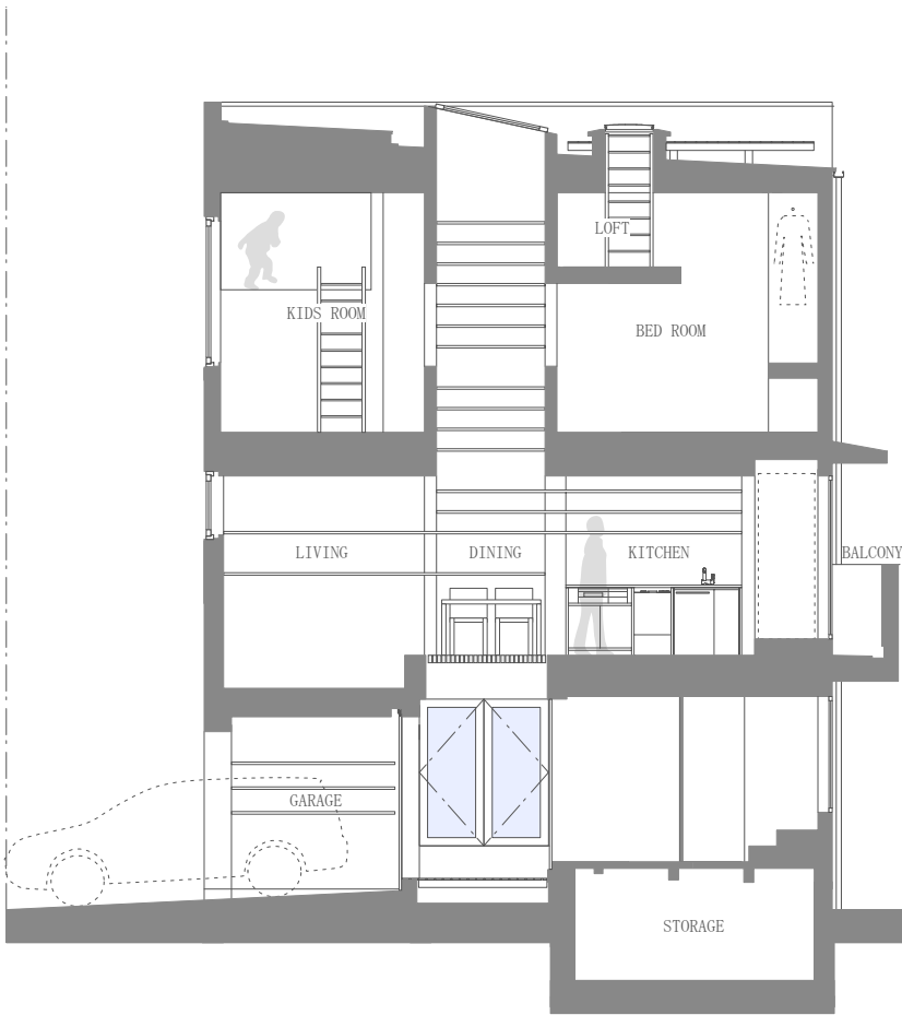
Section X-X' S=1:100
