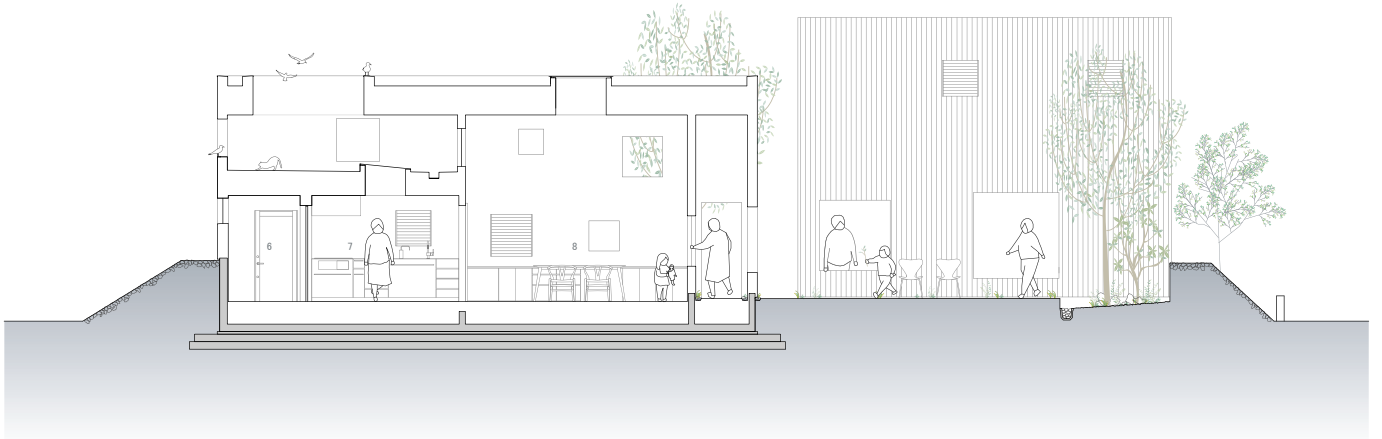
typeA section
