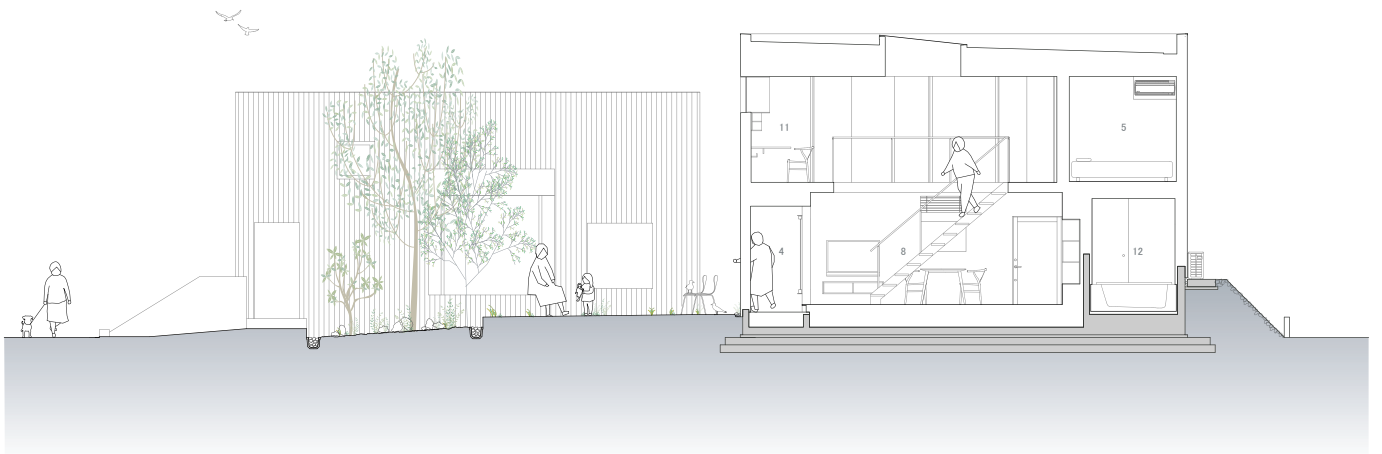
typeB section
