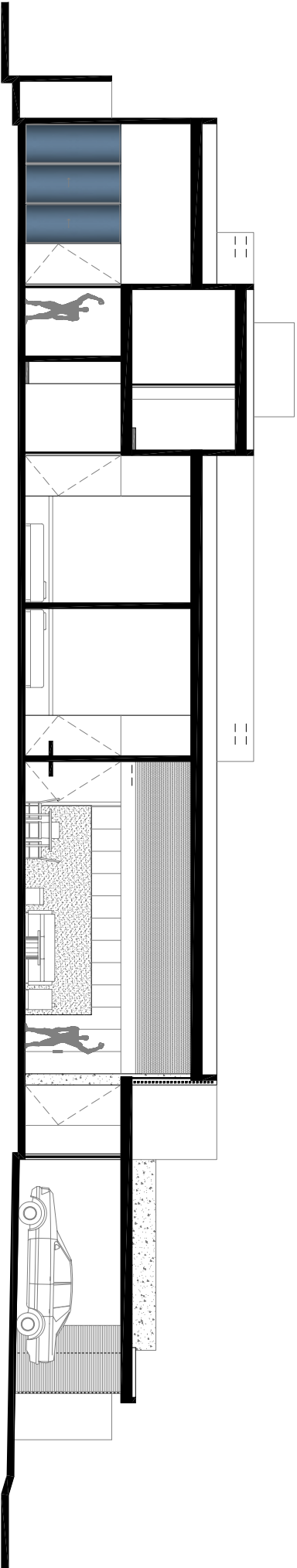
SECTION Y-Y' 0 1 2 3 5
