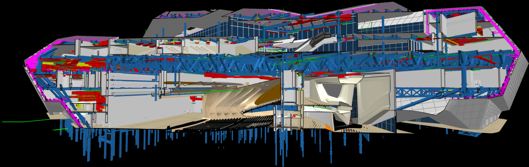
Nanjing International Youth Cultural Centre BIM MODEL - Section
