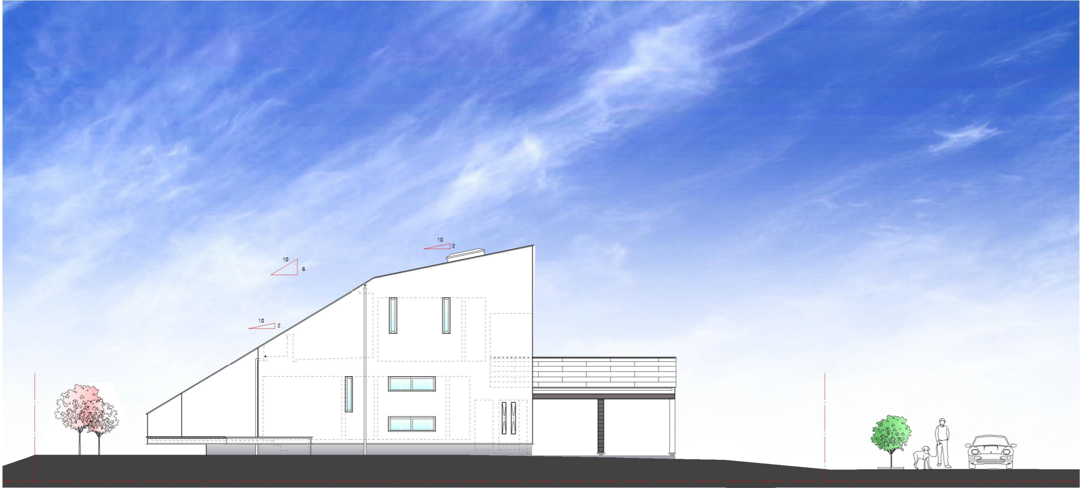
North Elevation
