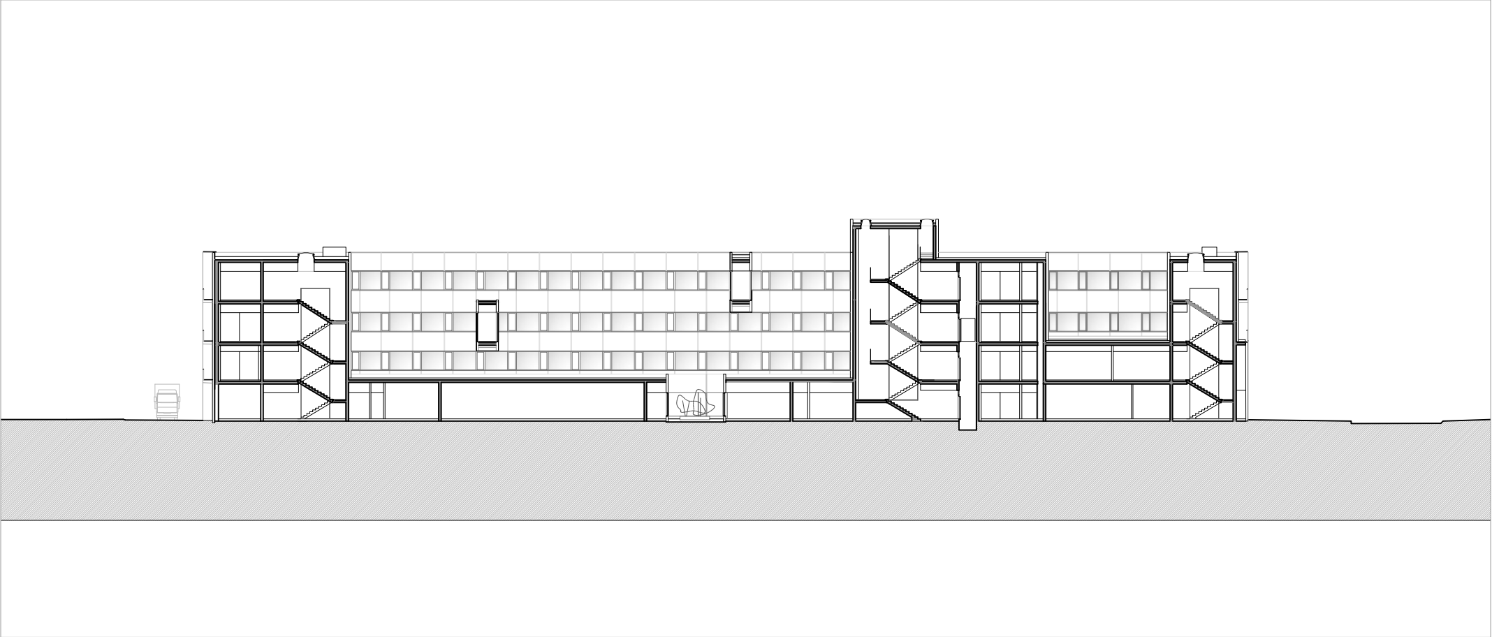
section aa
