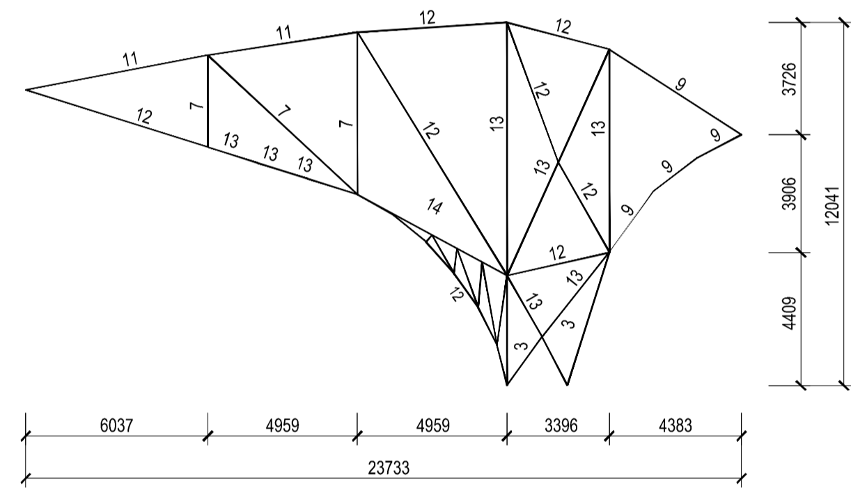
Radial Main Truss 7 - (E) Elevation Projection Diagram
