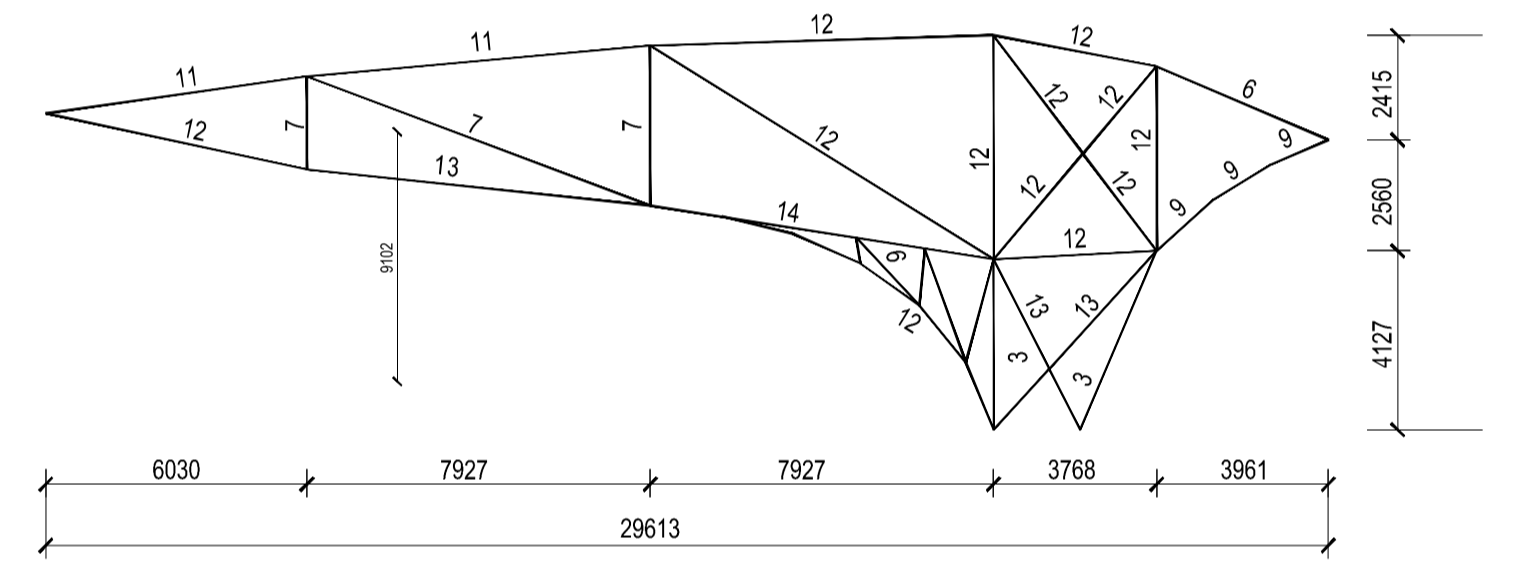
Radial Main Truss 9 - (E) Elevation Projection Diagram
