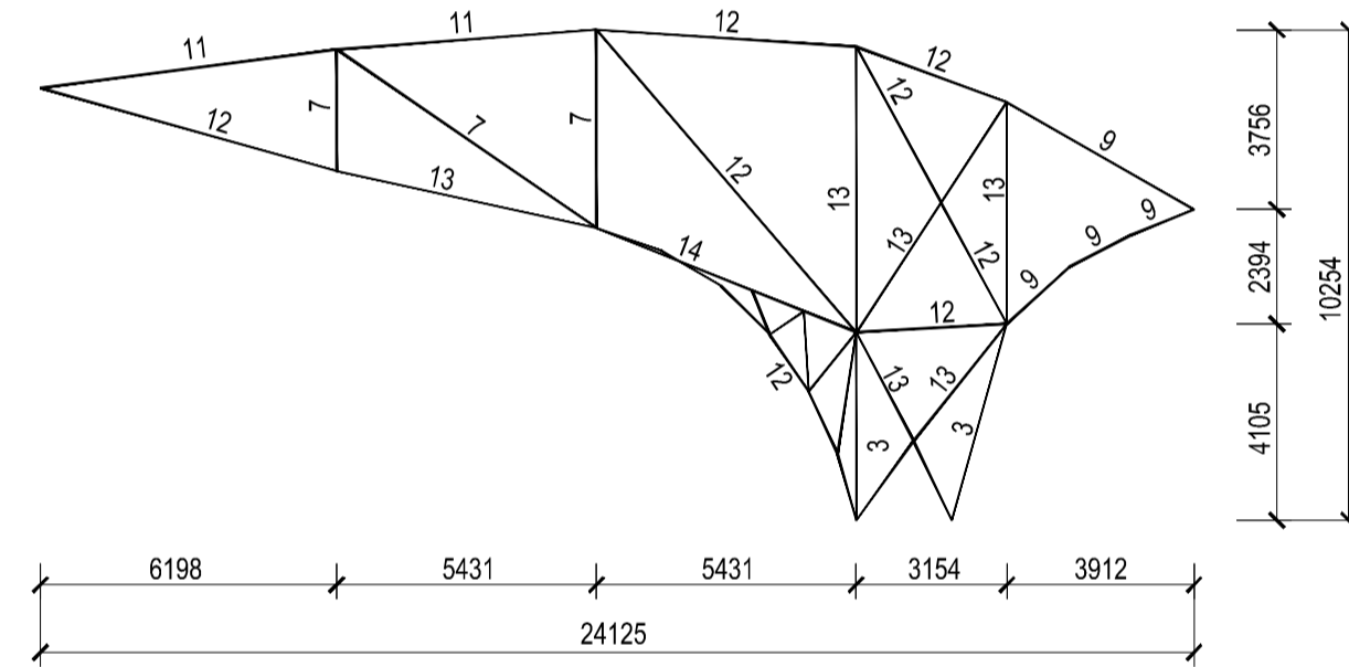
Radial Main Truss 8 - (E) Elevation Projection Diagram
