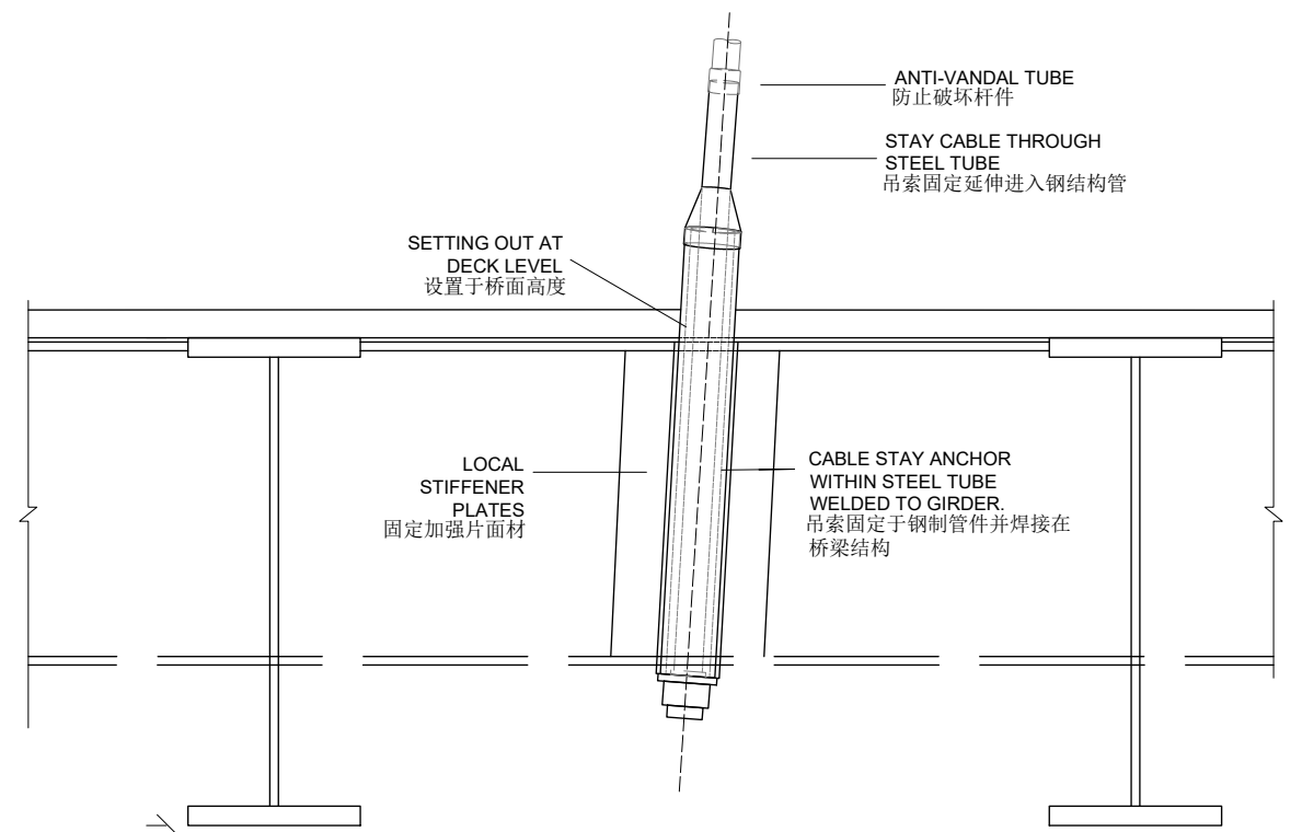
Chengdu Jiangxi River Bridge Typical Anchorage Detail 0 1m 2m
