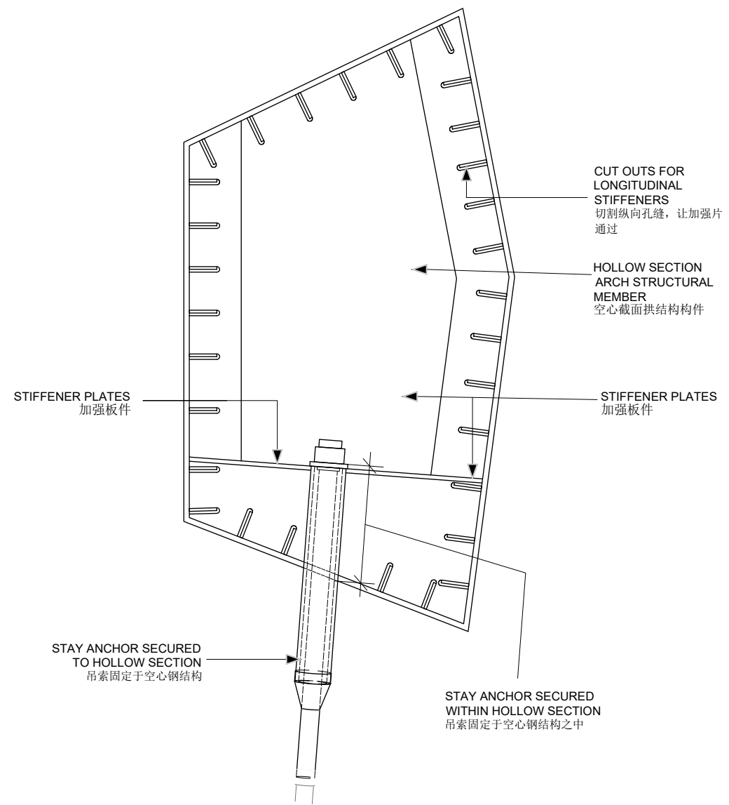
Chengdu Jiangxi River Bridge Typical Stay Anchorage At Arc 0 1m 2m
